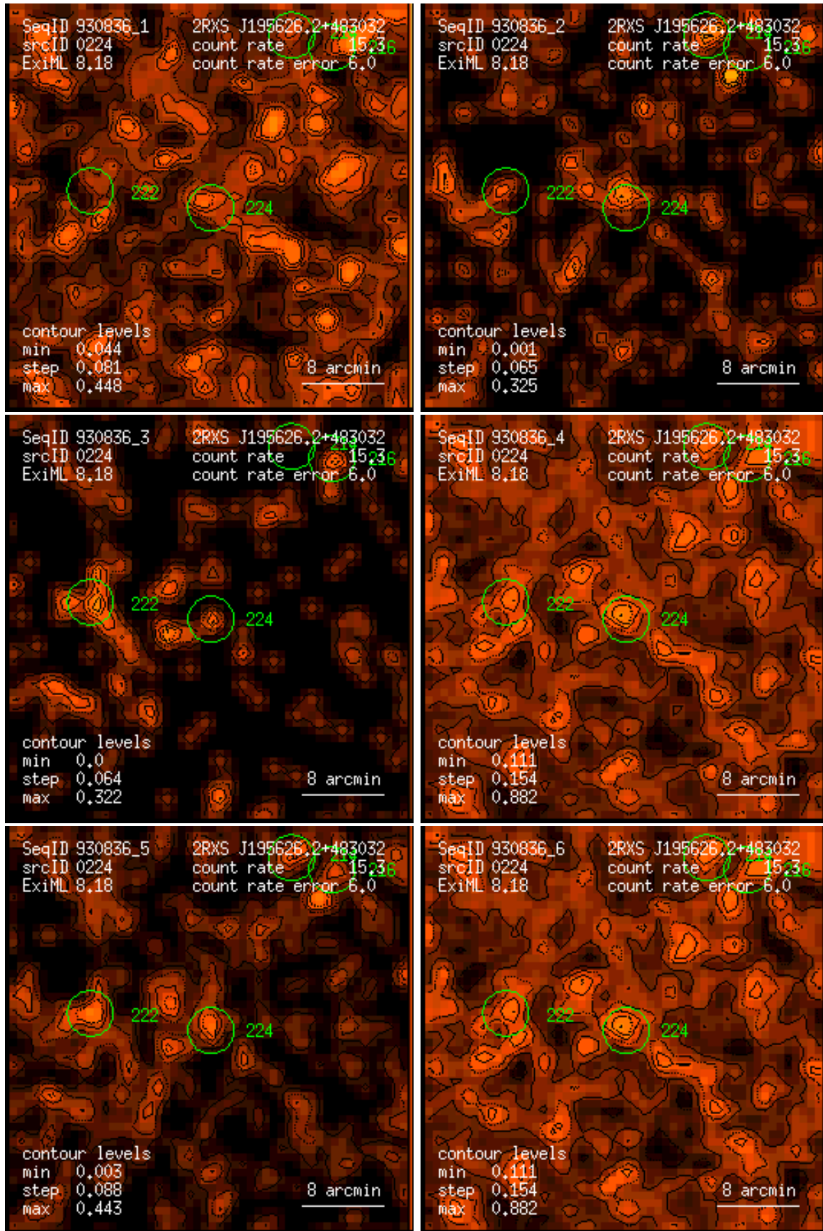
Figure 224: RASS 930836: detection 0224: band rate images, Gaussian filter: (1) PSPC channels 11 – 41, (2) 52 – 90, (3) 91 – 201, (4) 11 – 235, (5) 52 – 201, (6) 11 – 201. Broad band rates in counts/ks. Band rate contour levels in counts/ks/arcmin 2 .
