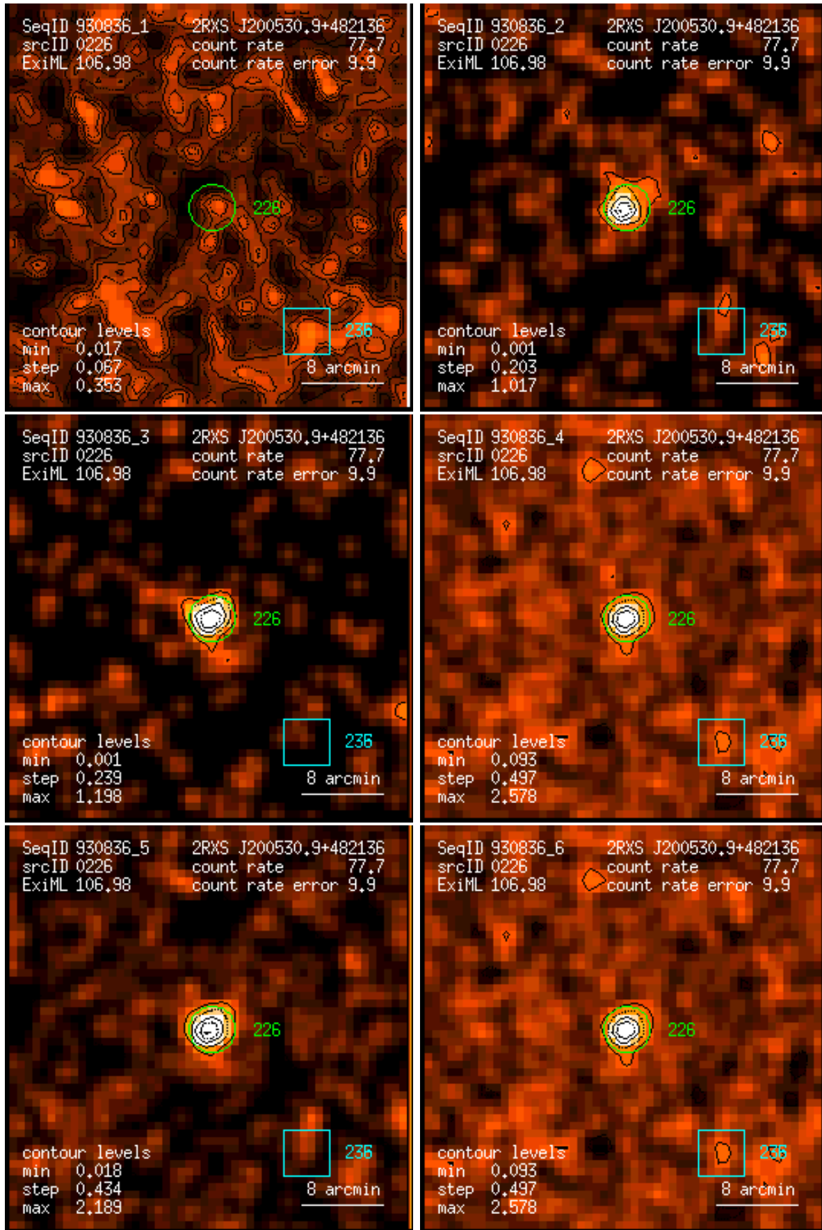
Figure 226: RASS 930836: detection 0226: band rate images, Gaussian filter: (1) PSPC channels 11 – 41, (2) 52 – 90, (3) 91 – 201, (4) 11 – 235, (5) 52 – 201, (6) 11 – 201. Broad band rates in counts/ks. Band rate contour levels in counts/ks/arcmin 2 .
