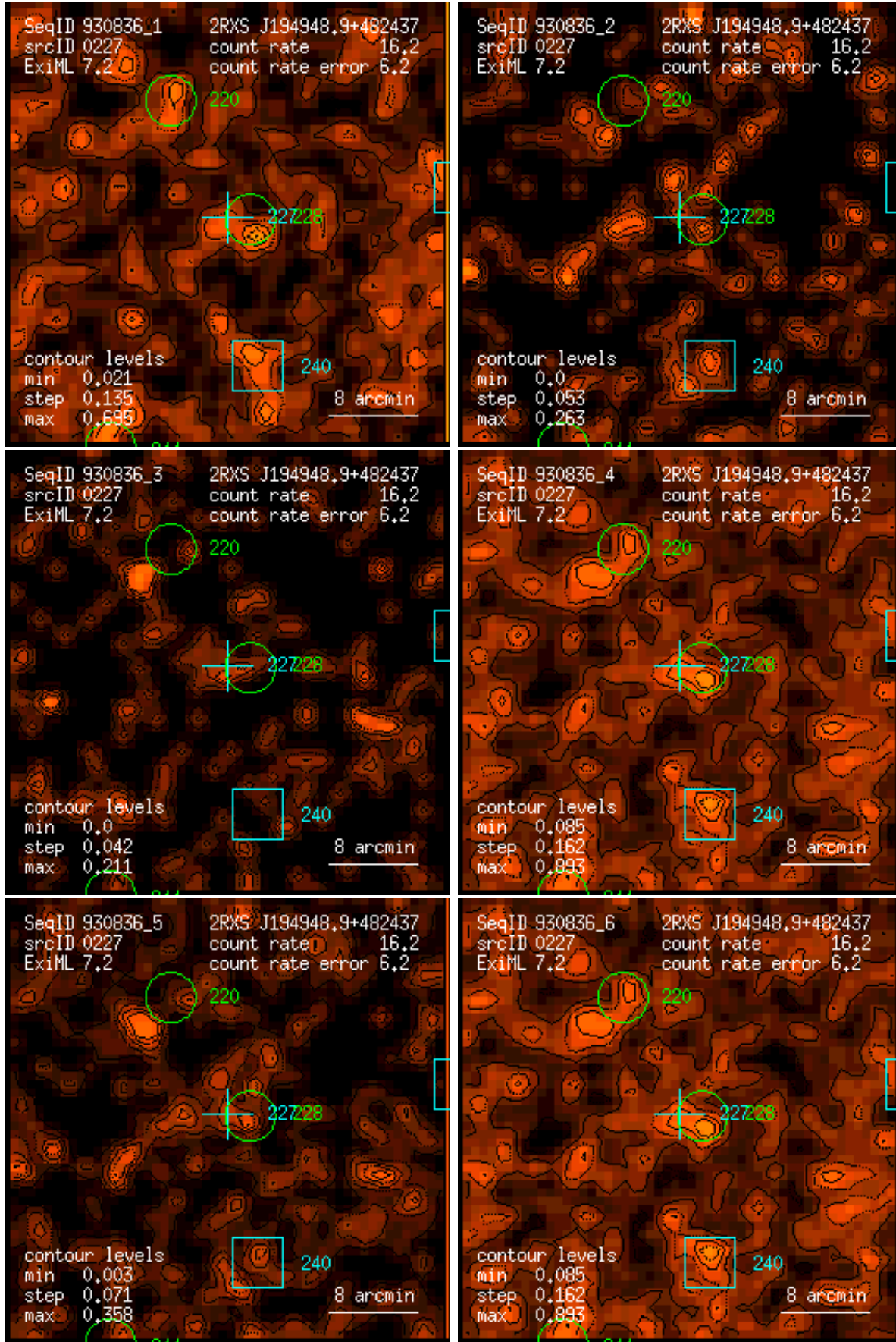
Figure 227: RASS 930836: detection 0227: band rate images, Gaussian filter: (1) PSPC channels 11 – 41, (2) 52 – 90, (3) 91 – 201, (4) 11 – 235, (5) 52 – 201, (6) 11 – 201. Broad band rates in counts/ks. Band rate contour levels in counts/ks/arcmin 2 .
