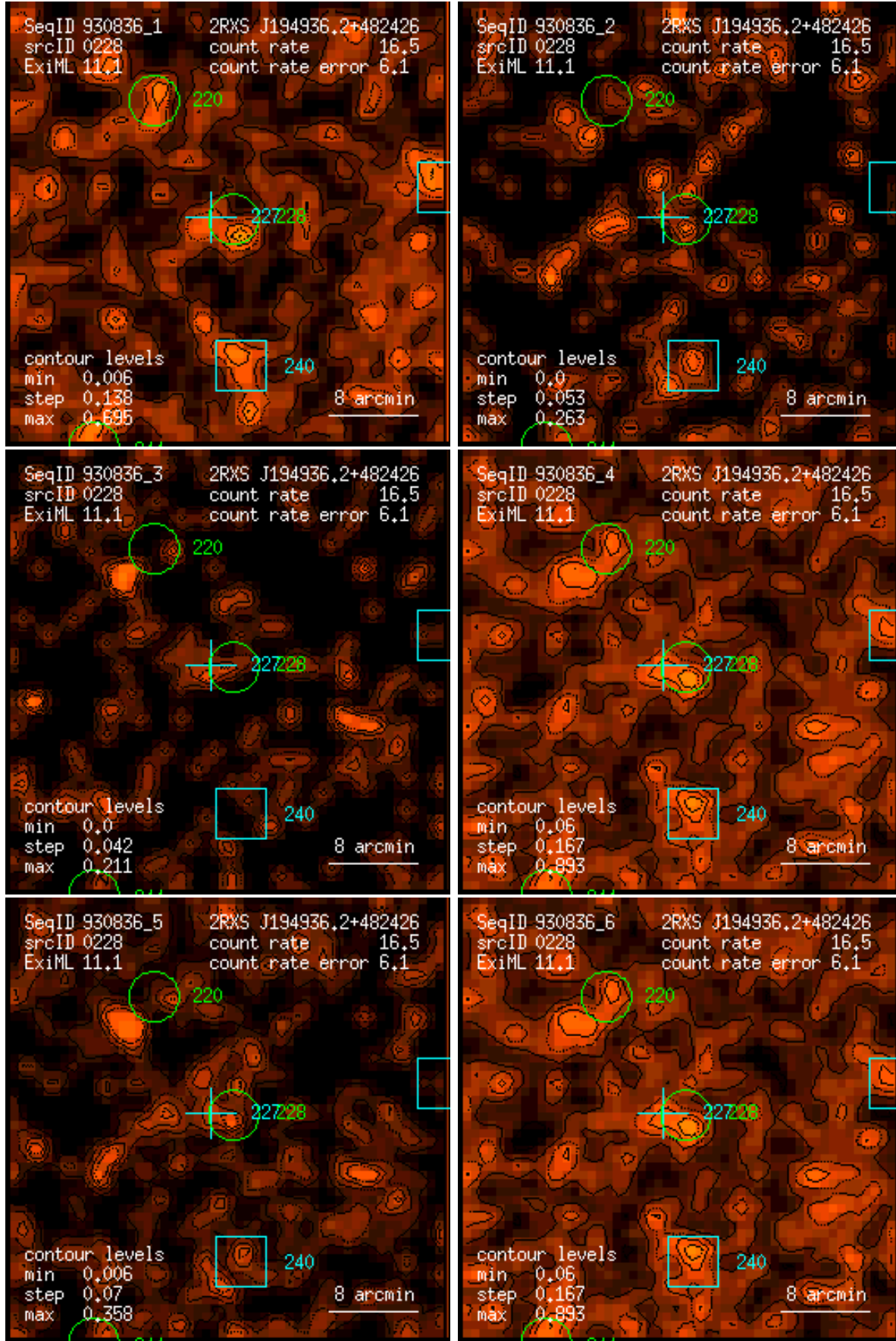
Figure 228: RASS 930836: detection 0228: band rate images, Gaussian filter: (1) PSPC channels 11 – 41, (2) 52 – 90, (3) 91 – 201, (4) 11 – 235, (5) 52 – 201, (6) 11 – 201. Broad band rates in counts/ks. Band rate contour levels in counts/ks/arcmin 2 .
