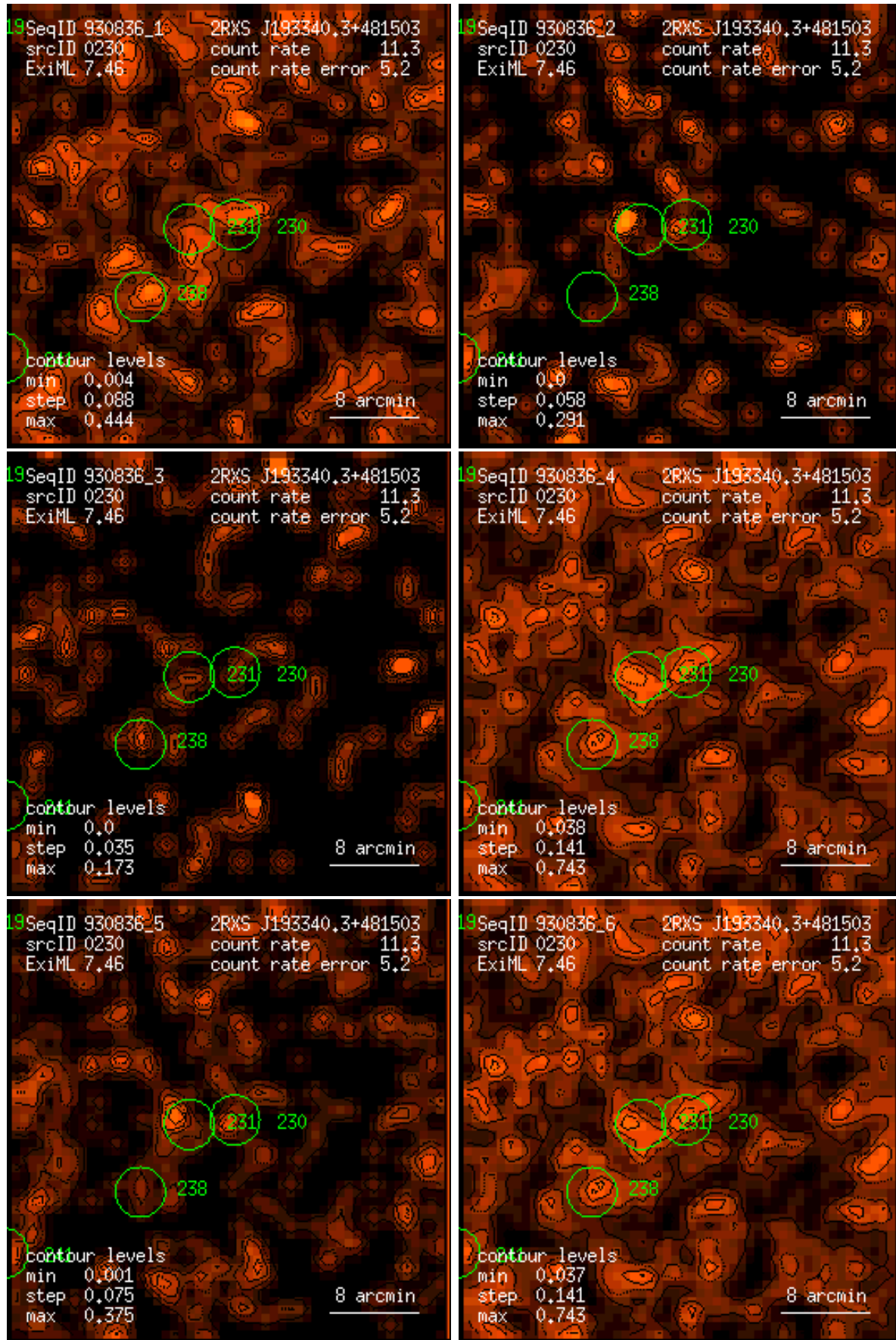
Figure 230: RASS 930836: detection 0230: band rate images, Gaussian filter: (1) PSPC channels 11 – 41, (2) 52 – 90, (3) 91 – 201, (4) 11 – 235, (5) 52 – 201, (6) 11 – 201. Broad band rates in counts/ks. Band rate contour levels in counts/ks/arcmin 2 .
