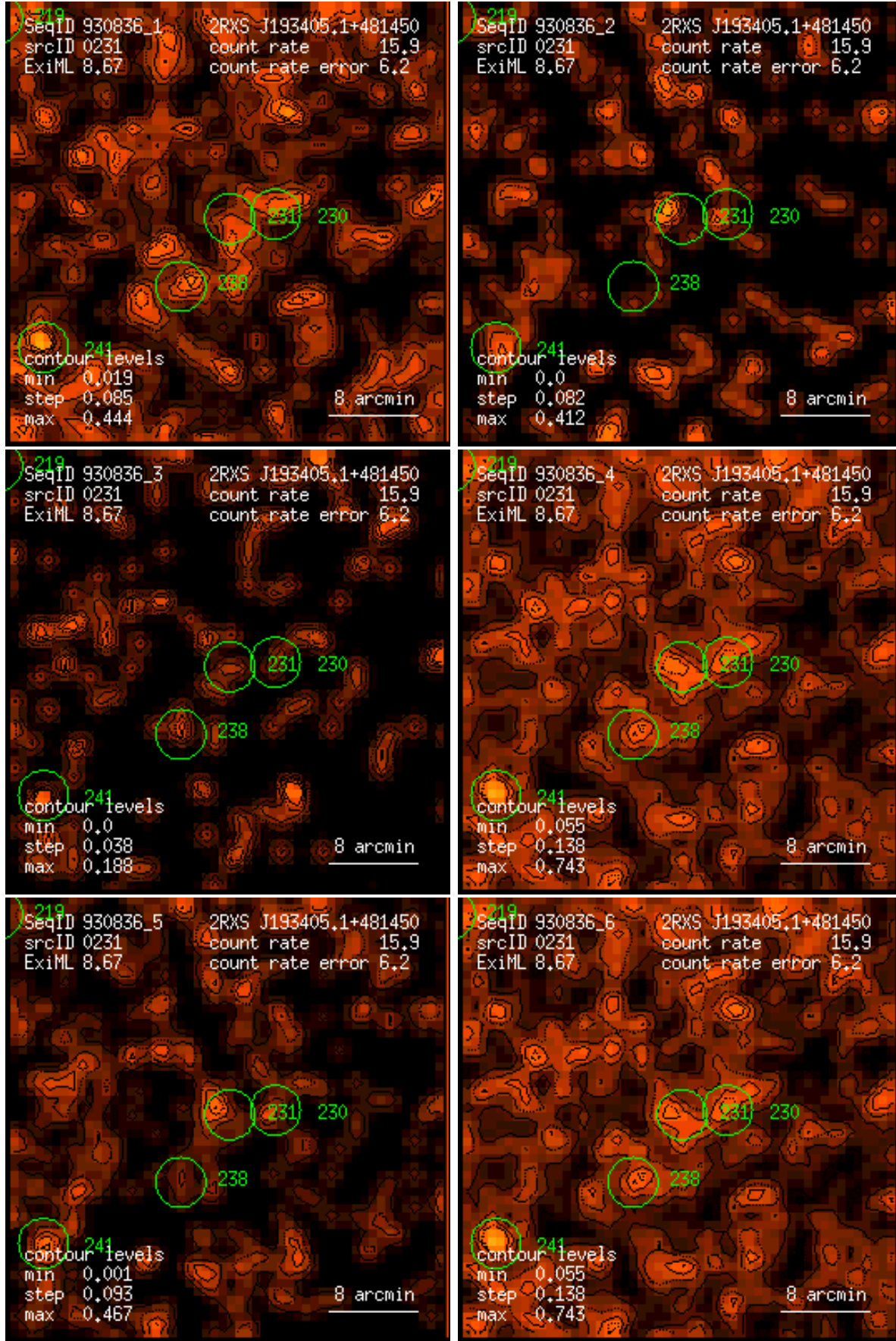
Figure 231: RASS 930836: detection 0231: band rate images, Gaussian filter: (1) PSPC channels 11 – 41, (2) 52 – 90, (3) 91 – 201, (4) 11 – 235, (5) 52 – 201, (6) 11 – 201. Broad band rates in counts/ks. Band rate contour levels in counts/ks/arcmin 2 .
