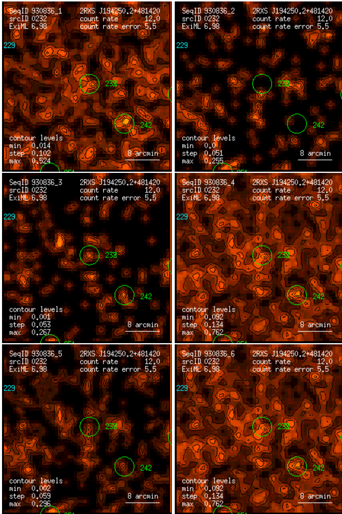
Figure 232: RASS 930836: detection 0232: band rate images, Gaussian filter: (1) PSPC channels 11 – 41, (2) 52 – 90, (3) 91 – 201, (4) 11 – 235, (5) 52 – 201, (6) 11 – 201. Broad band rates in counts/ks. Band rate contour levels in counts/ks/arcmin 2 .
