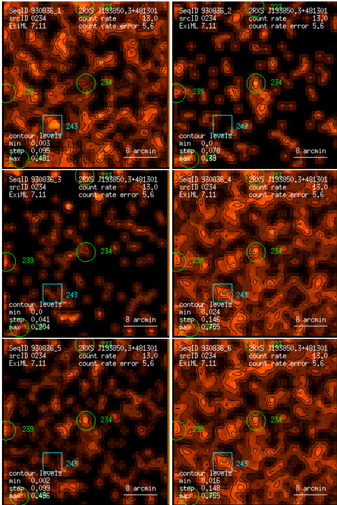
Figure 234: RASS 930836: detection 0234: band rate images, Gaussian filter: (1) PSPC channels 11 – 41, (2) 52 – 90, (3) 91 – 201, (4) 11 – 235, (5) 52 – 201, (6) 11 – 201. Broad band rates in counts/ks. Band rate contour levels in counts/ks/arcmin 2 .
