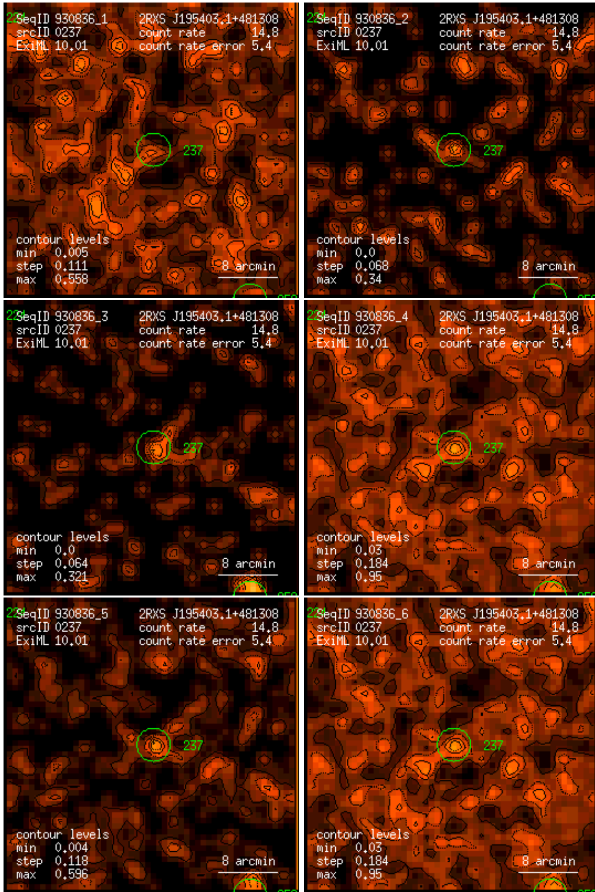
Figure 237: RASS 930836: detection 0237: band rate images, Gaussian filter: (1) PSPPC channels 11 – 41, (2) 52 – 90, (3) 91 – 201, (4) 11 – 235, (5) 52 – 201, (6) 11 – 201. Broad band rates in counts/ks. Band rate contour levels in counts/ks/arcmin 2 .
