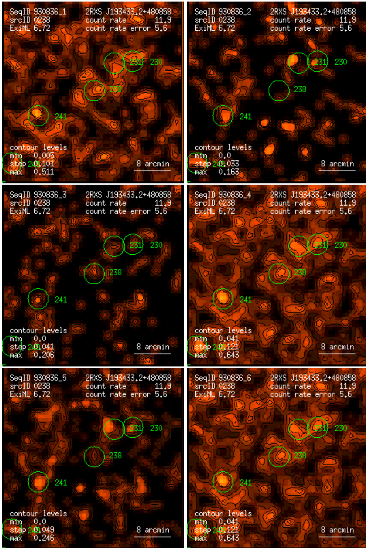
Figure 238: RASS 930836: detection 0238: band rate images, Gaussian filter: (1) PSPC channels 11 – 41, (2) 52 – 90, (3) 91 – 201, (4) 11 – 235, (5) 52 – 201, (6) 11 – 201. Broad band rates in counts/ks. Band rate contour levels in counts/ks/arcmin 2 .
