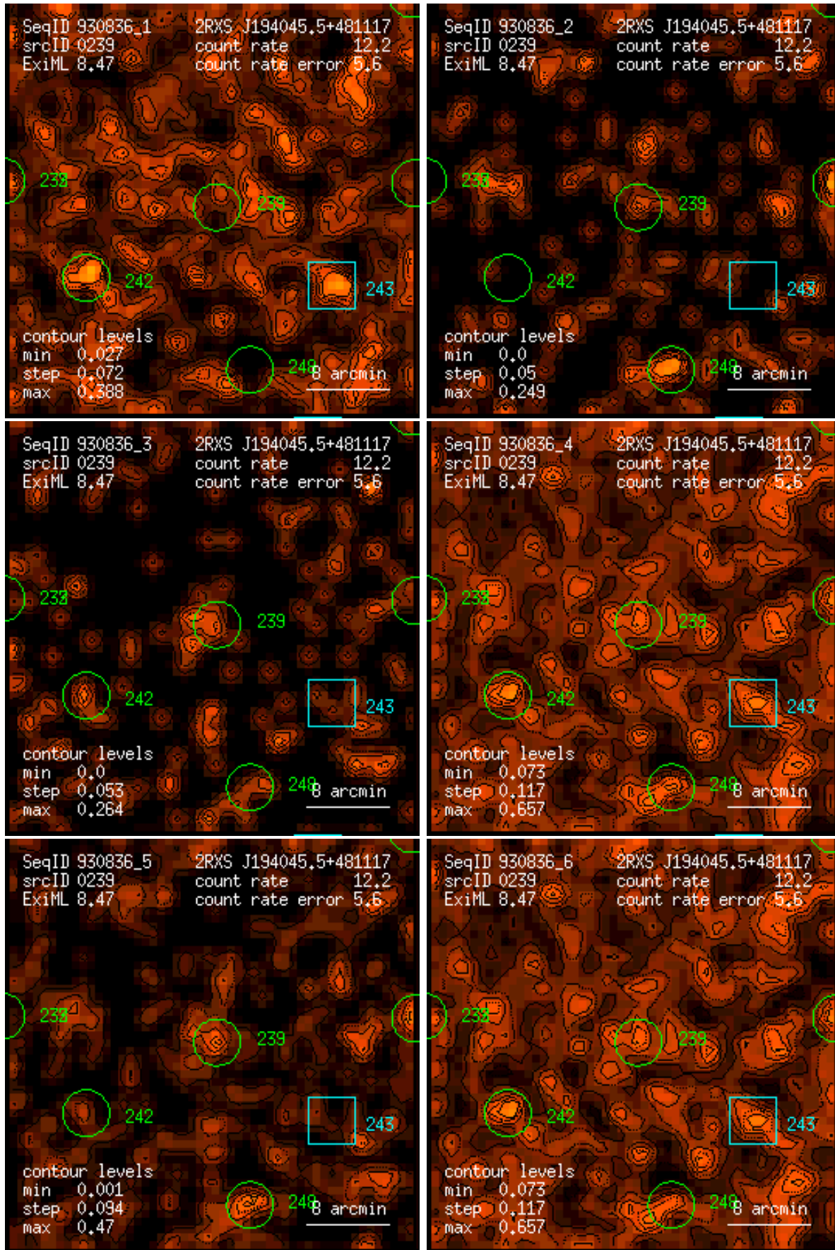
Figure 239: RASS 930836: detection 0239: band rate images, Gaussian filter: (1) PSPC channels 11 – 41, (2) 52 – 90, (3) 91 – 201, (4) 11 – 235, (5) 52 – 201, (6) 11 – 201. Broad band rates in counts/ks. Band rate contour levels in counts/ks/arcmin 2 .
