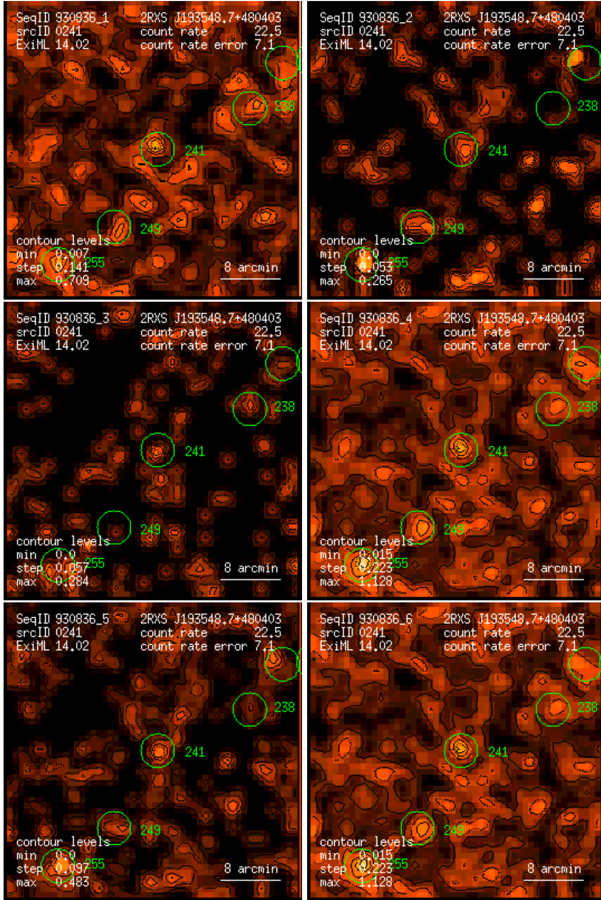
Figure 241: RASS 930836: detection 0241: band rate images, Gaussian filter: (1) PSPC channels 11 – 41, (2) 52 – 90, (3) 91 – 201, (4) 11 – 235, (5) 52 – 201, (6) 11 – 201. Broad band rates in counts/ks. Band rate contour levels in counts/ks/arcmin 2 .
