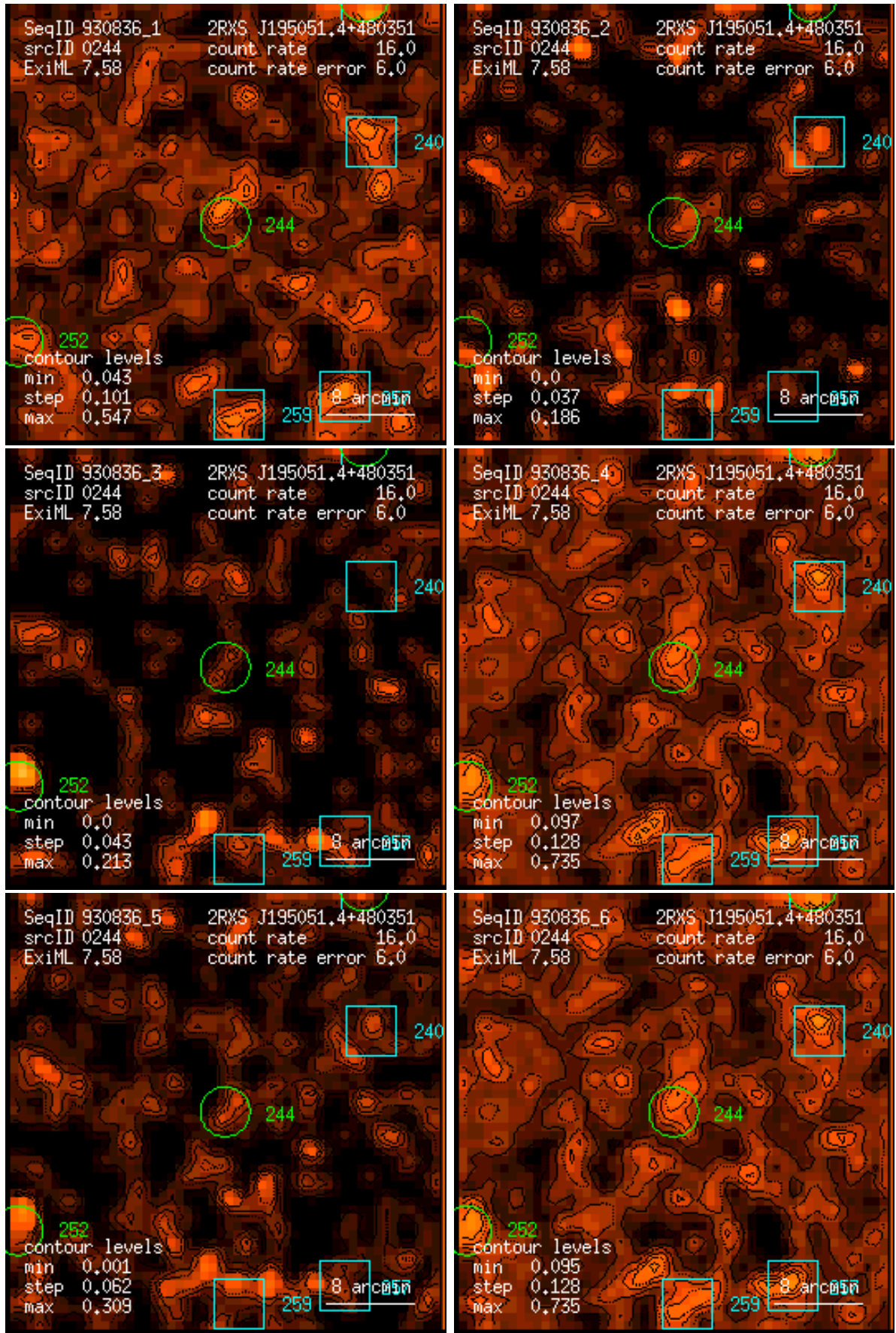
Figure 244: RASS 930836: detection 0244: band rate images, Gaussian filter: (1) PSPC channels 11 – 41, (2) 52 – 90, (3) 91 – 201, (4) 11 – 235, (5) 52 – 201, (6) 11 – 201. Broad band rates in counts/ks. Band rate contour levels in counts/ks/arcmin 2 .
