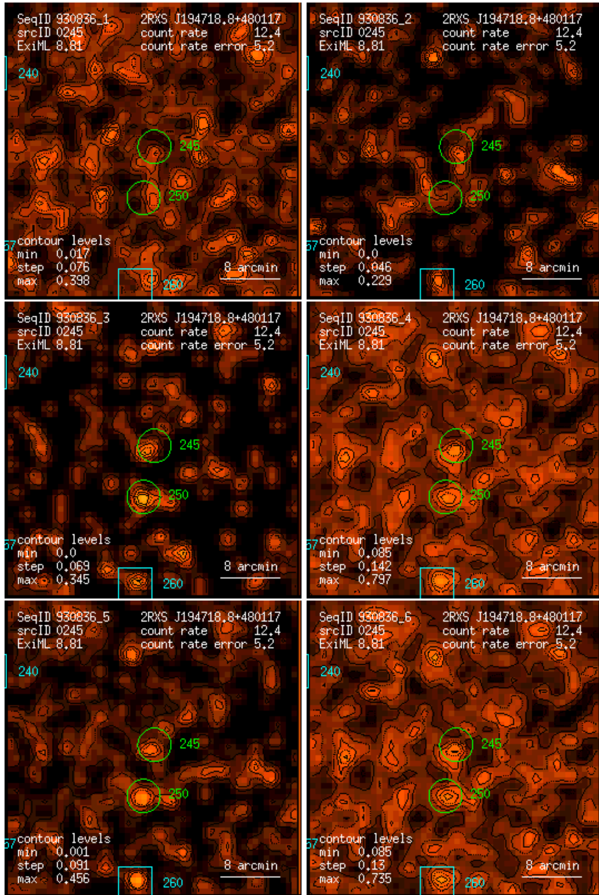
Figure 245: RASS 930836: detection 0245: band rate images, Gaussian filter: (1) PSPC channels 11 – 41, (2) 52 – 90, (3) 91 – 201, (4) 11 – 235, (5) 52 – 201, (6) 11 – 201. Broad band rates in counts/ks. Band rate contour levels in counts/ks/arcmin 2 .
