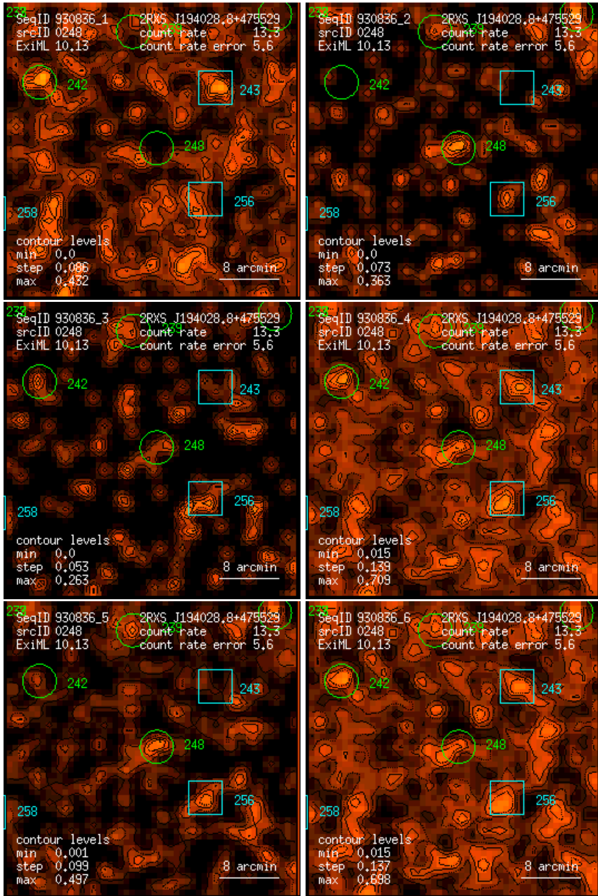
Figure 248: RASS 930836: detection 0248: band rate images, Gaussian filter: (1) PSPC channels 11 – 41, (2) 52 – 90, (3) 91 – 201, (4) 11 – 235, (5) 52 – 201, (6) 11 – 201. Broad band rates in counts/ks. Band rate contour levels in counts/ks/arcmin 2 .
