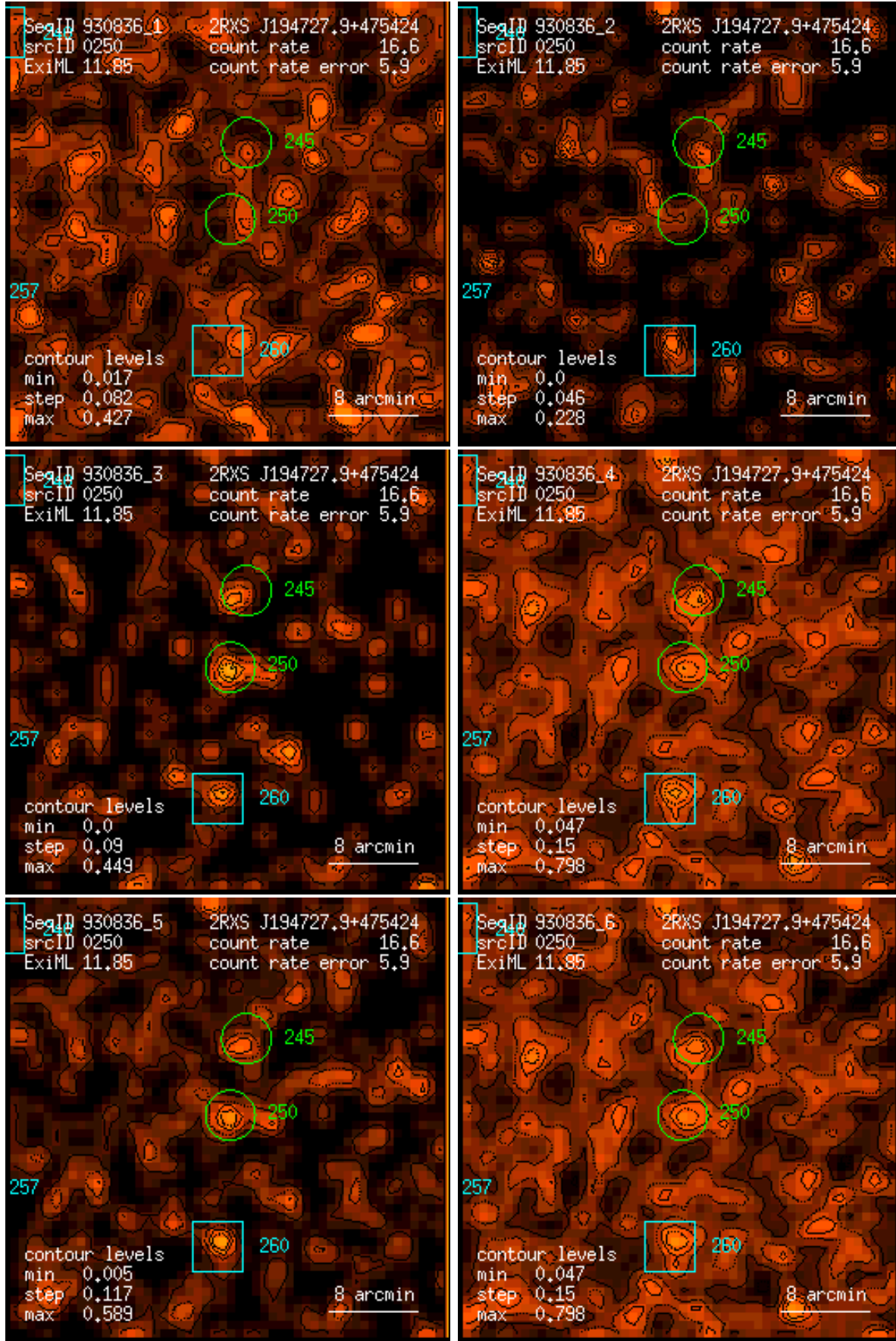
Figure 250: RASS 930836: detection 0250: band rate images, Gaussian filter: (1) PSPC channels 11 – 41, (2) 52 – 90, (3) 91 – 201, (4) 11 – 235, (5) 52 – 201, (6) 11 – 201. Broad band rates in counts/ks. Band rate contour levels in counts/ks/arcmin 2 .
