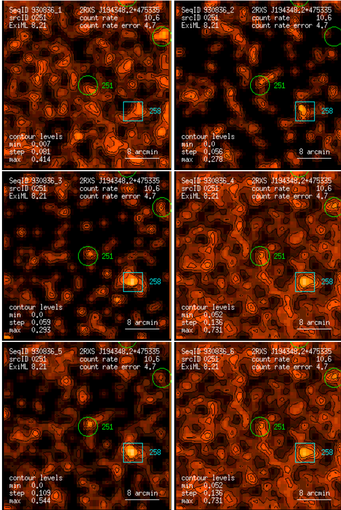
Figure 251: RASS 930836: detection 0251: band rate images, Gaussian filter: (1) PSPC channels 11 – 41, (2) 52 – 90, (3) 91 – 201, (4) 11 – 235, (5) 52 – 201, (6) 11 – 201. Broad band rates in counts/ks. Band rate contour levels in counts/ks/arcmin 2 .
