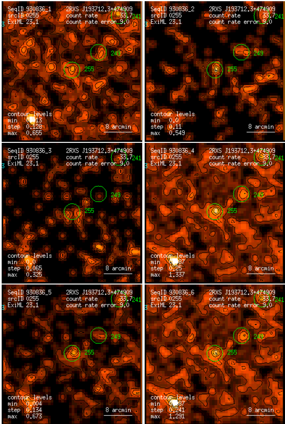
Figure 255: RASS 930836: detection 0255: band rate images, Gaussian filter: (1) PSPC channels 11 – 41, (2) 52 – 90, (3) 91 – 201, (4) 11 – 235, (5) 52 – 201, (6) 11 – 201. Broad band rates in counts/ks. Band rate contour levels in counts/ks/arcmin 2 .
