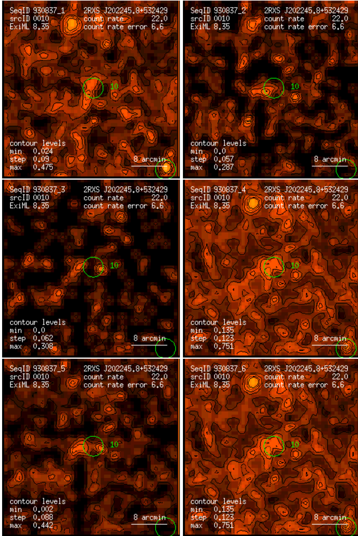
Figure 10: RASS 930837: detection 0010: band rate images, Gaussian filter: (1) PSPC channels 11 – 41, (2) 52 – 90, (3) 91 – 201, (4) 11 – 235, (5) 52 – 201, (6) 11 – 201. Broad band rates in counts/ks. Band rate contour levels in counts/ks/arcmin 2 .
