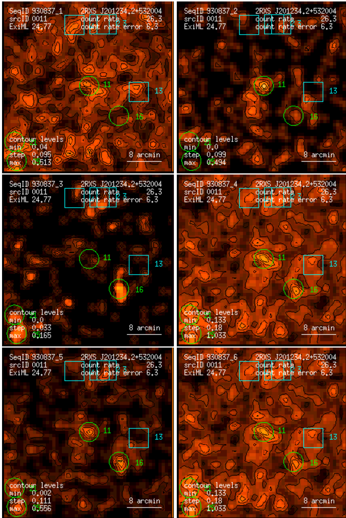
Figure 11: RASS 930837: detection 0011: band rate images, Gaussian filter: (1) PSPC channels 11 – 41, (2) 52 – 90, (3) 91 – 201, (4) 11 – 235, (5) 52 – 201, (6) 11 – 201. Broad band rates in counts/ks. Band rate contour levels in counts/ks/arcmin 2 .
