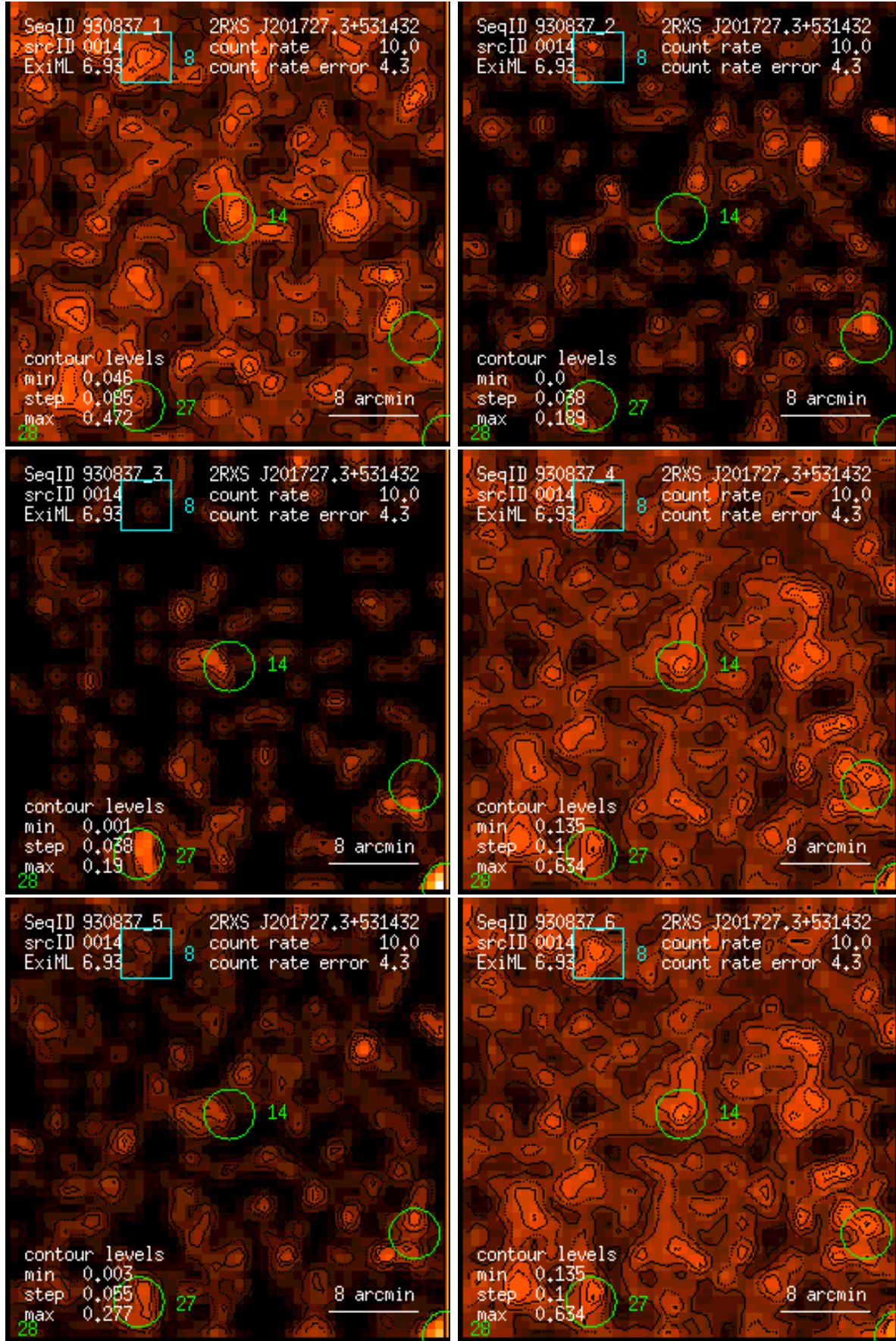
Figure 14: RASS 930837: detection 0014: band rate images, Gaussian filter: (1) PSPC channels 11 – 41, (2) 52 – 90, (3) 91 – 201, (4) 11 – 235, (5) 52 – 201, (6) 11 – 201. Broad band rates in counts/ks. Band rate contour levels in counts/ks/arcmin 2 .
