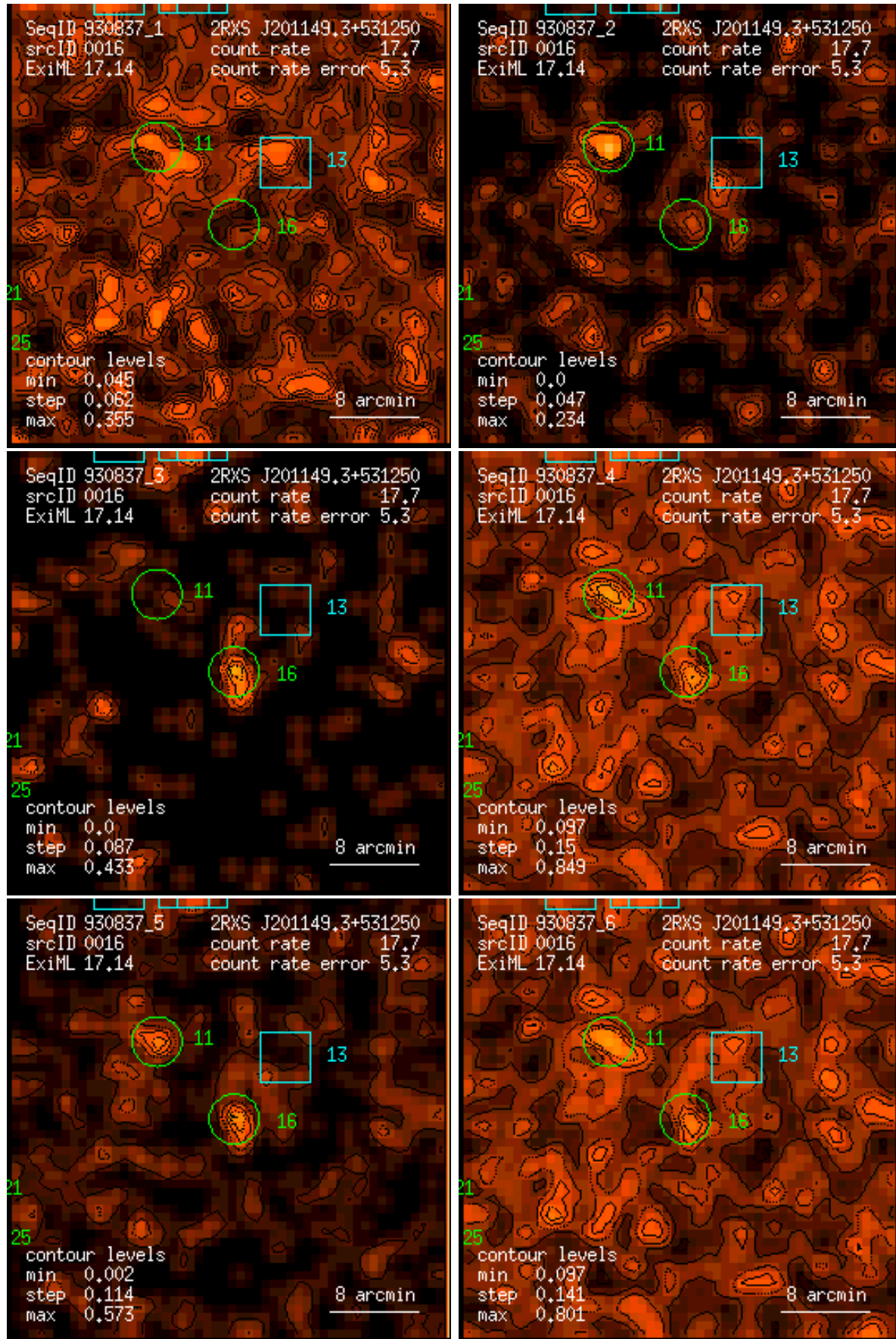
Figure 16: RASS 930837: detection 0016: band rate images, Gaussian filter: (1) PSPC channels 11 – 41, (2) 52 – 90, (3) 91 – 201, (4) 11 – 235, (5) 52 – 201, (6) 11 – 201. Broad band rates in counts/ks. Band rate contour levels in counts/ks/arcmin 2 .
