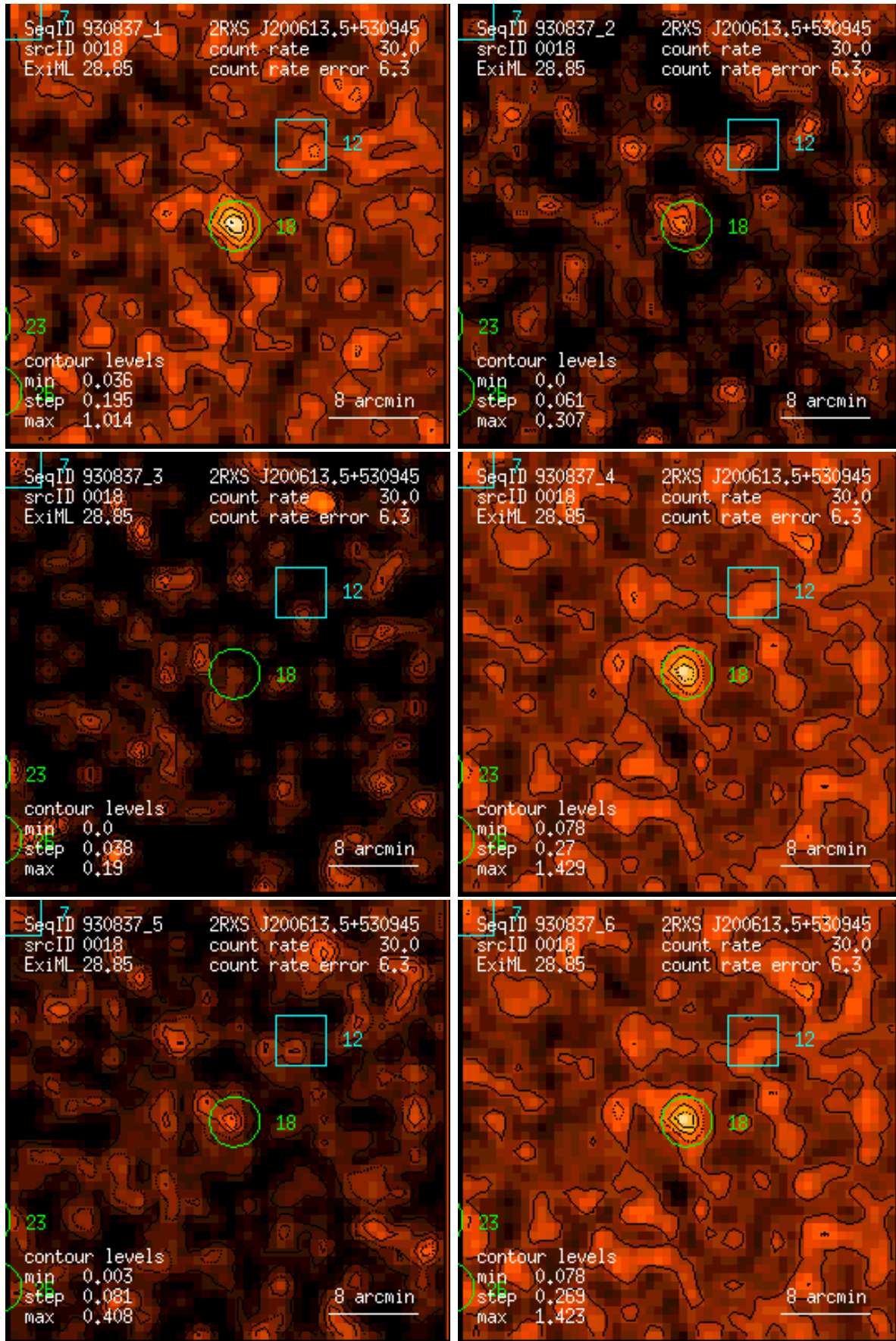
Figure 18: RASS 930837: detection 0018: band rate images, Gaussian filter: (1) PSPC channels 11 – 41, (2) 52 – 90, (3) 91 – 201, (4) 11 – 235, (5) 52 – 201, (6) 11 – 201. Broad band rates in counts/ks. Band rate contour levels in counts/ks/arcmin 2 .
