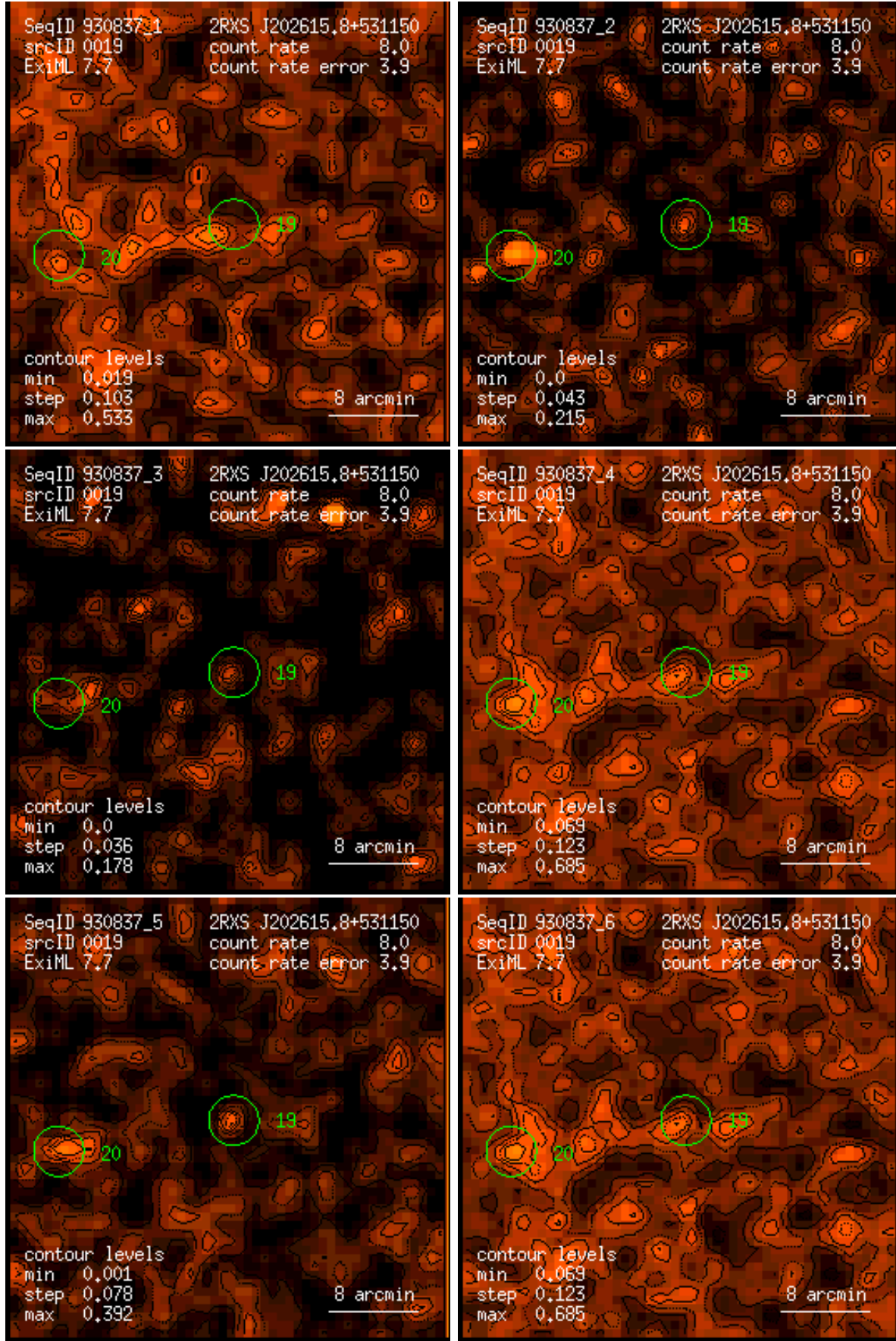
Figure 19: RASS 930837: detection 0019: band rate images, Gaussian filter: (1) PSPC channels 11 – 41, (2) 52 – 90, (3) 91 – 201, (4) 11 – 235, (5) 52 – 201, (6) 11 – 201. Broad band rates in counts/ks. Band rate contour levels in counts/ks/arcmin 2 .
