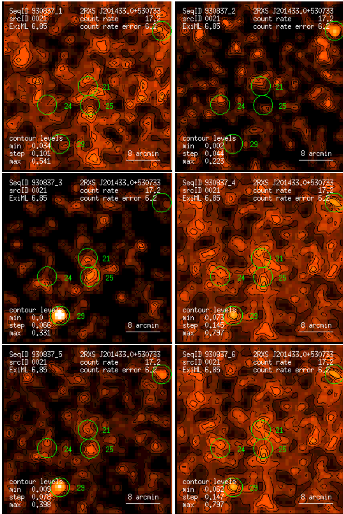
Figure 21: RASS 930837: detection 0021: band rate images, Gaussian filter: (1) PSPC channels 11 – 41, (2) 52 – 90, (3) 91 – 201, (4) 11 – 235, (5) 52 – 201, (6) 11 – 201. Broad band rates in counts/ks. Band rate contour levels in counts/ks/arcmin 2 .
