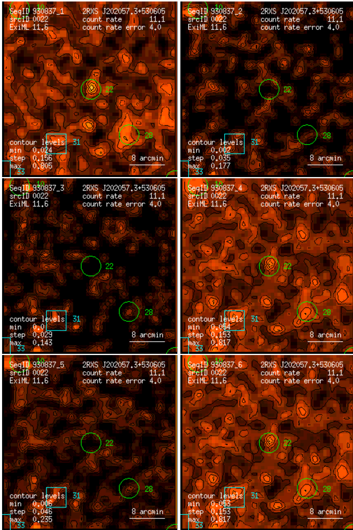
Figure 22: RASS 930837: detection 0022: band rate images, Gaussian filter: (1) PSPC channels 11 – 41, (2) 52 – 90, (3) 91 – 201, (4) 11 – 235, (5) 52 – 201, (6) 11 – 201. Broad band rates in counts/ks. Band rate contour levels in counts/ks/arcmin 2 .
