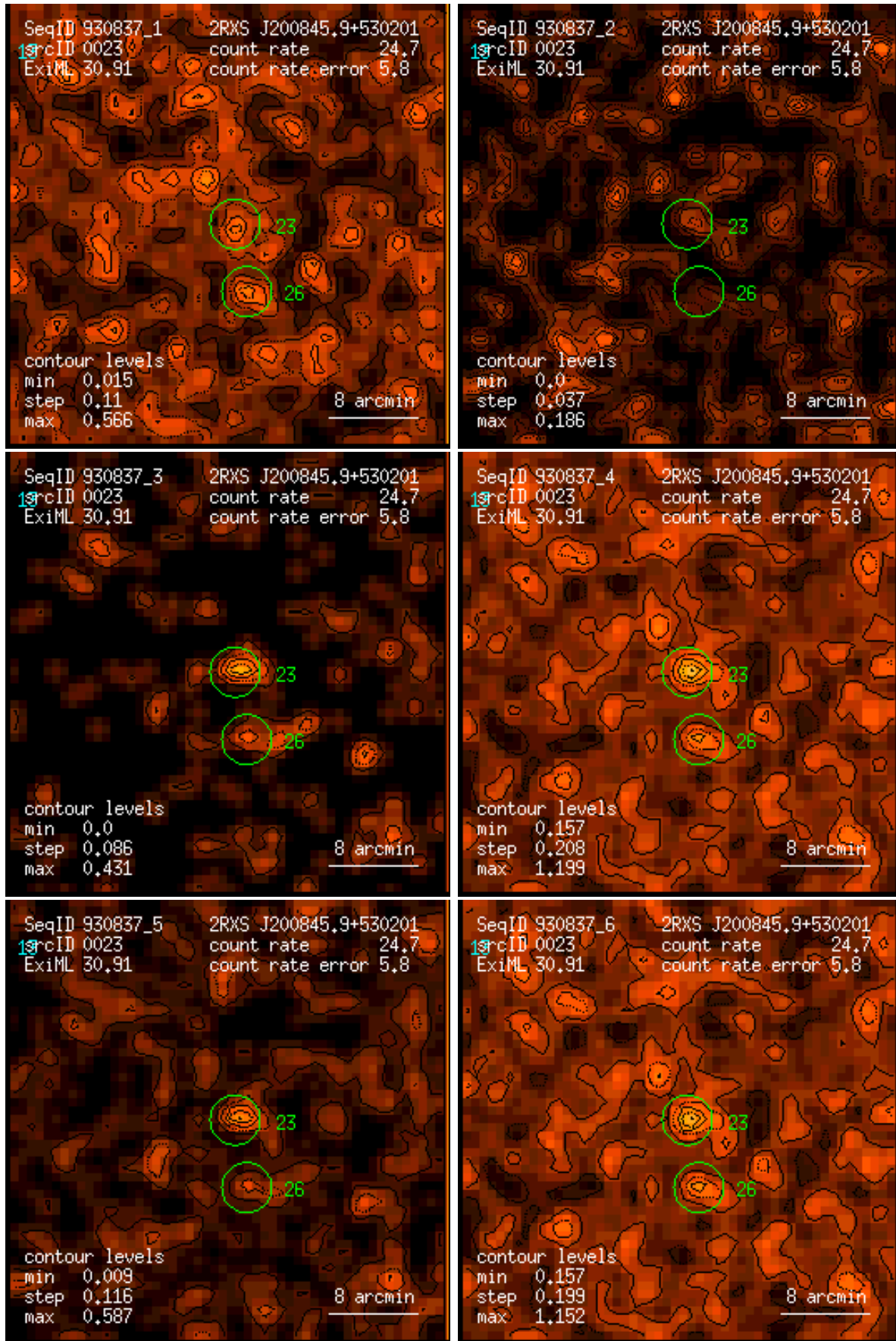
Figure 23: RASS 930837: detection 0023: band rate images, Gaussian filter: (1) PSPC channels 11 – 41, (2) 52 – 90, (3) 91 – 201, (4) 11 – 235, (5) 52 – 201, (6) 11 – 201. Broad band rates in counts/ks. Band rate contour levels in counts/ks/arcmin 2 .
