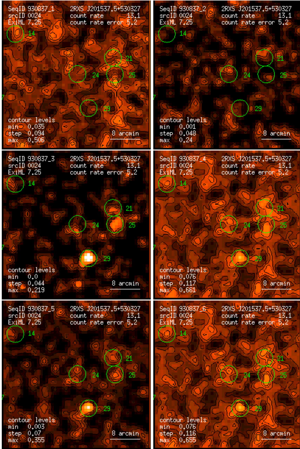
Figure 24: RASS 930837: detection 0024: band rate images, Gaussian filter: (1) PSPC channels 11 – 41, (2) 52 – 90, (3) 91 – 201, (4) 11 – 235, (5) 52 – 201, (6) 11 – 201. Broad band rates in counts/ks. Band rate contour levels in counts/ks/arcmin 2 .
