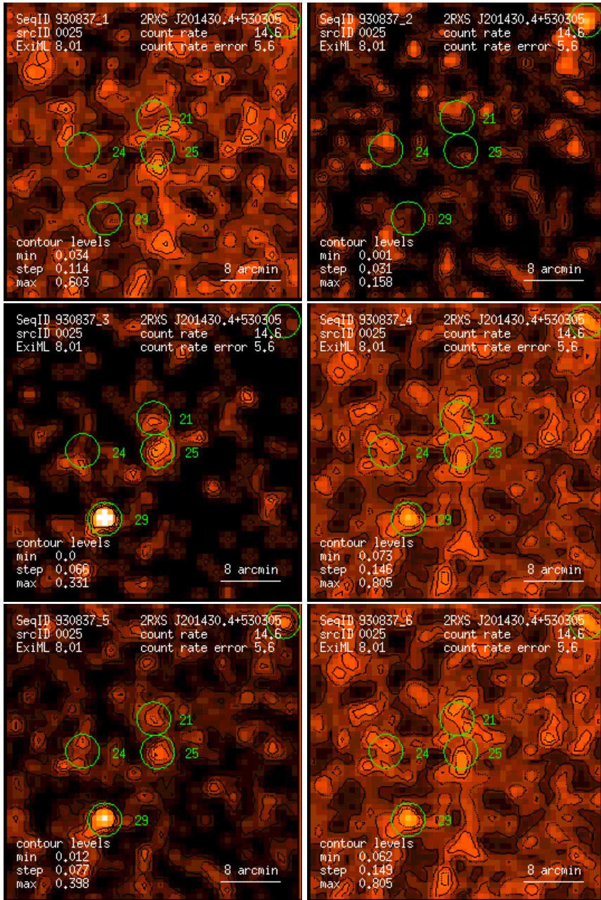
Figure 25: RASS 930837: detection 0025: band rate images, Gaussian filter: (1) PSPC channels 11 – 41, (2) 52 – 90, (3) 91 – 201, (4) 11 – 235, (5) 52 – 201, (6) 11 – 201. Broad band rates in counts/ks. Band rate contour levels in counts/ks/arcmin 2 .
