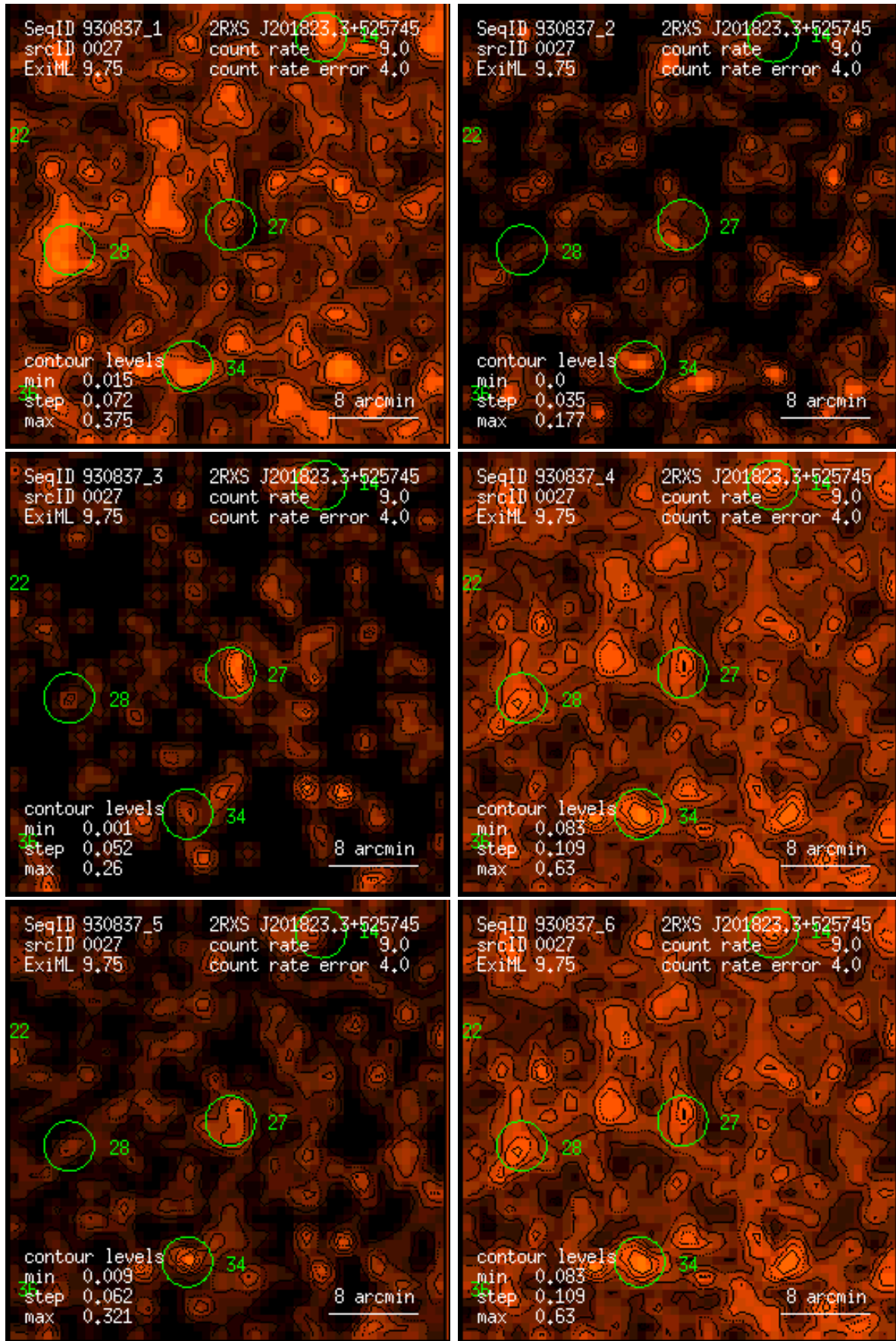
Figure 27: RASS 930837: detection 0027: band rate images, Gaussian filter: (1) PSPC channels 11 – 41, (2) 52 – 90, (3) 91 – 201, (4) 11 – 235, (5) 52 – 201, (6) 11 – 201. Broad band rates in counts/ks. Band rate contour levels in counts/ks/arcmin 2 .
