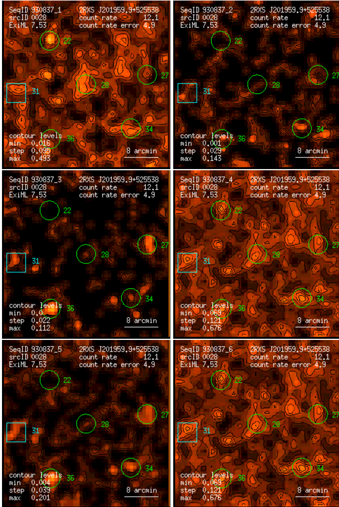
Figure 28: RASS 930837: detection 0028: band rate images, Gaussian filter: (1) PSPC channels 11 – 41, (2) 52 – 90, (3) 91 – 201, (4) 11 – 235, (5) 52 – 201, (6) 11 – 201. Broad band rates in counts/ks. Band rate contour levels in counts/ks/arcmin 2 .
