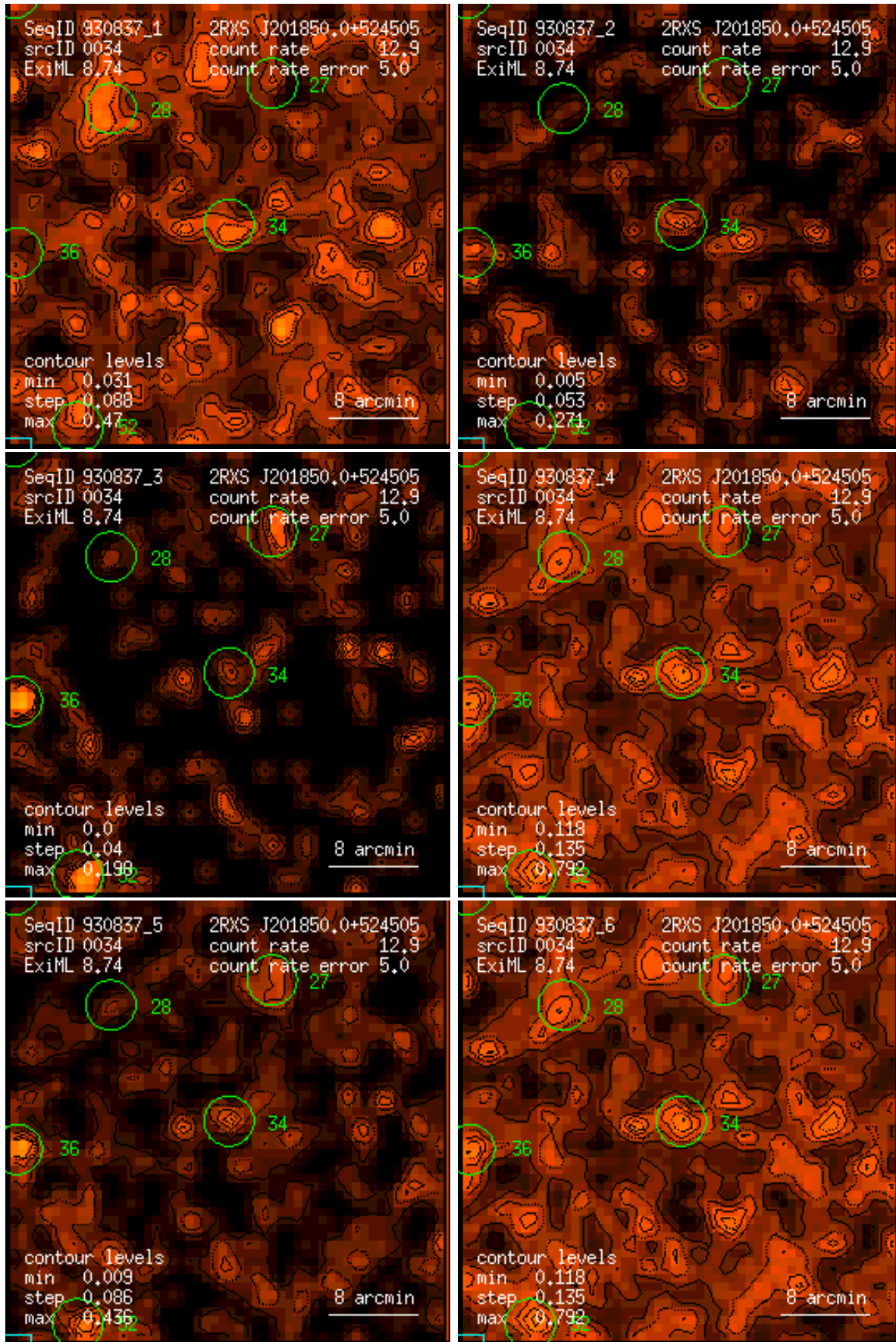
Figure 34: RASS 930837: detection 0034: band rate images, Gaussian filter: (1) PSPC channels 11 – 41, (2) 52 – 90, (3) 91 – 201, (4) 11 – 235, (5) 52 – 201, (6) 11 – 201. Broad band rates in counts/ks. Band rate contour levels in counts/ks/arcmin 2 .
