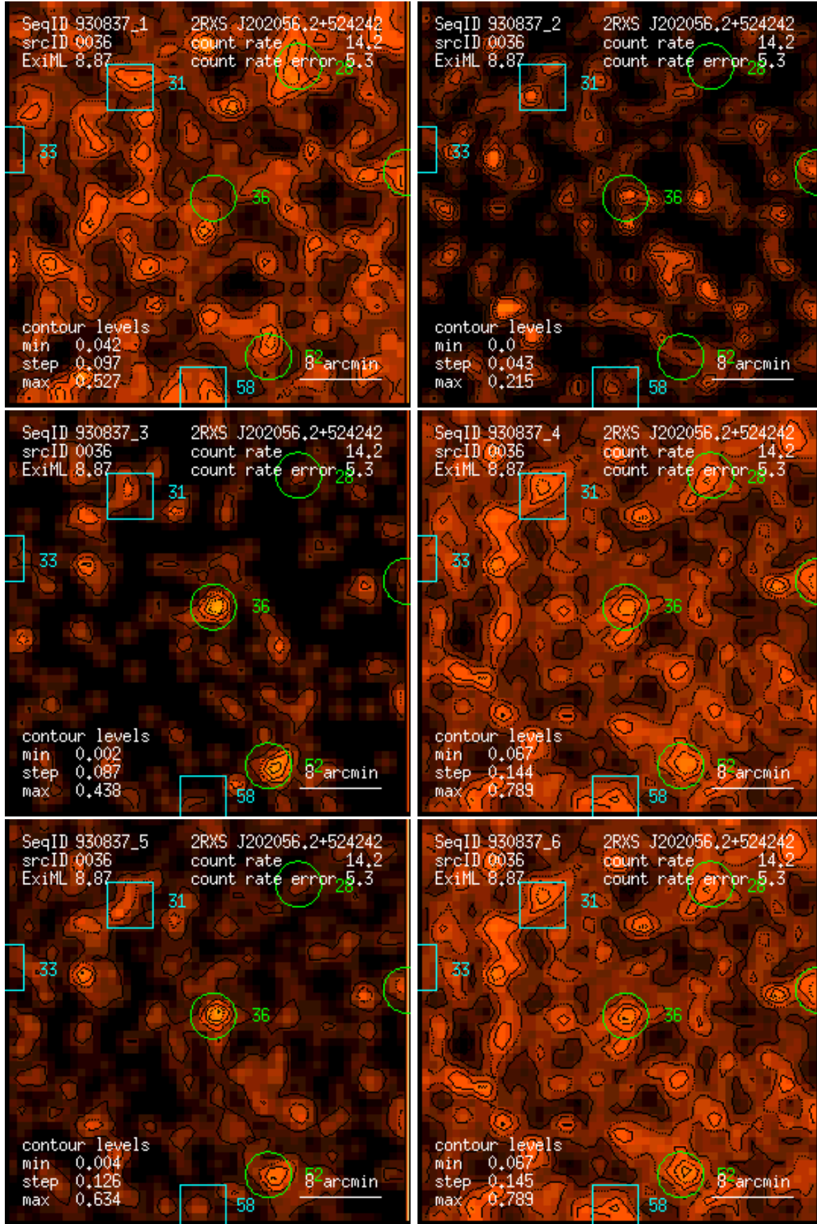
Figure 36: RASS 930837: detection 0036: band rate images, Gaussian filter: (1) PSPC channels 11 – 41, (2) 52 – 90, (3) 91 – 201, (4) 11 – 235, (5) 52 – 201, (6) 11 – 201. Broad band rates in counts/ks. Band rate contour levels in counts/ks/arcmin 2 .
