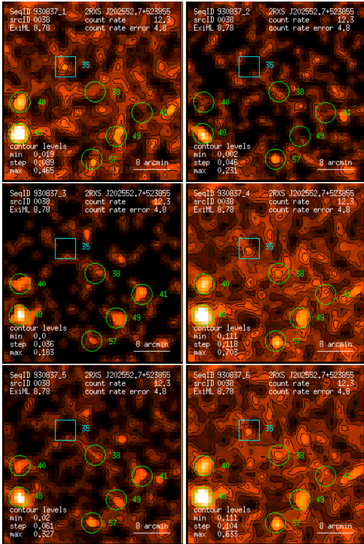
Figure 38: RASS 930837: detection 0038: band rate images, Gaussian filter: (1) PSPC channels 11 – 41, (2) 52 – 90, (3) 91 – 201, (4) 11 – 235, (5) 52 – 201, (6) 11 – 201. Broad band rates in counts/ks. Band rate contour levels in counts/ks/arcmin 2 .
