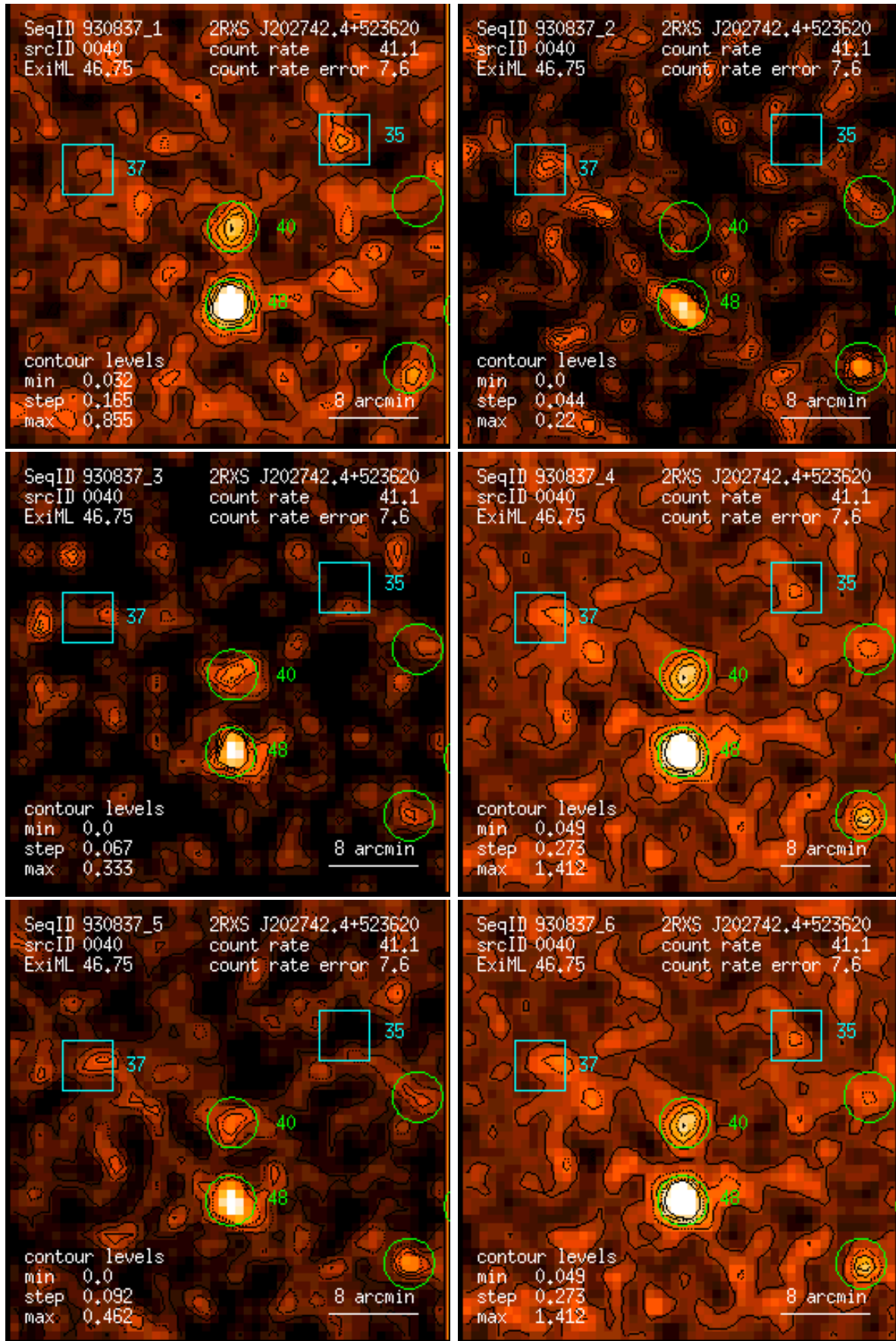
Figure 40: RASS 930837: detection 0040: band rate images, Gaussian filter: (1) PSPC channels 11 – 41, (2) 52 – 90, (3) 91 – 201, (4) 11 – 235, (5) 52 – 201, (6) 11 – 201. Broad band rates in counts/ks. Band rate contour levels in counts/ks/arcmin 2 .
