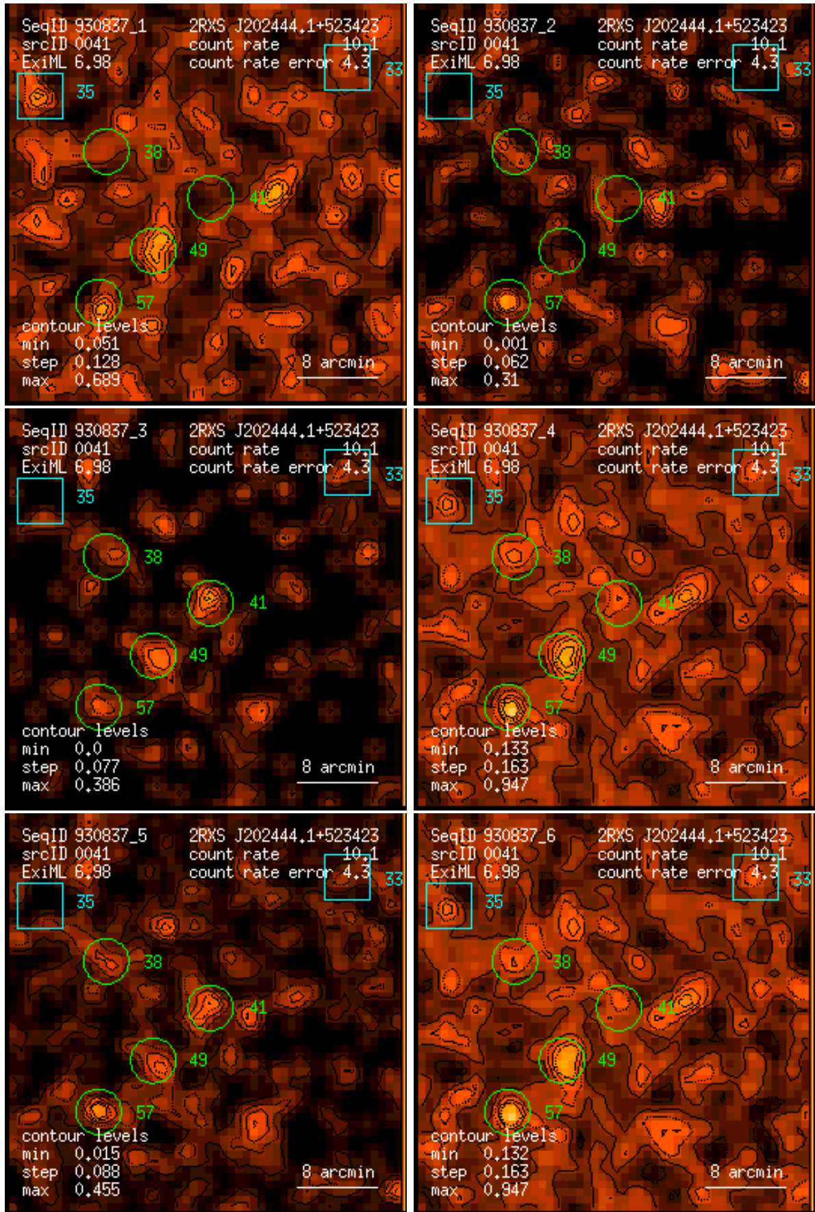
Figure 41: RASS 930837: detection 0041: band rate images, Gaussian filter: (1) PSPC channels 11 – 41, (2) 52 – 90, (3) 91 – 201, (4) 11 – 235, (5) 52 – 201, (6) 11 – 201. Broad band rates in counts/ks. Band rate contour levels in counts/ks/arcmin 2 .
