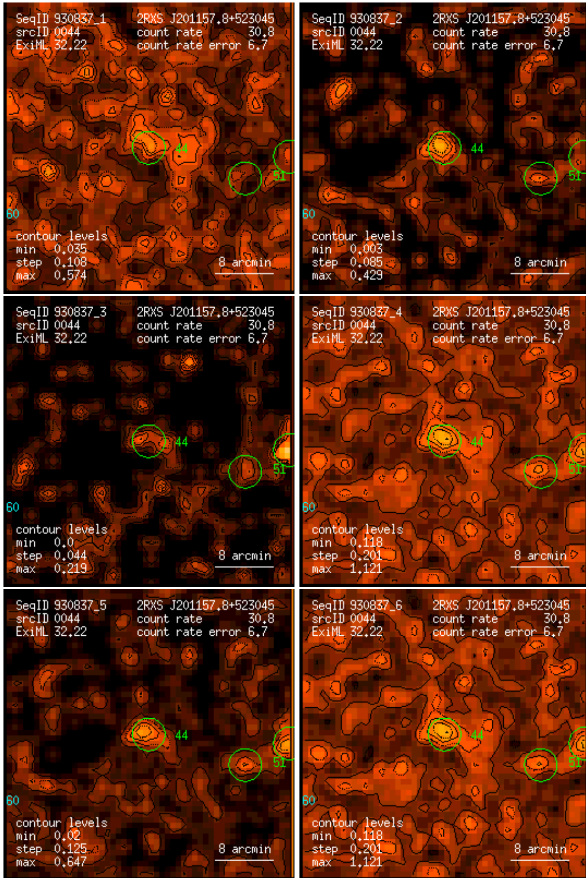
Figure 44: RASS 930837: detection 0044: band rate images, Gaussian filter: (1) PSPC channels 11 – 41, (2) 52 – 90, (3) 91 – 201, (4) 11 – 235, (5) 52 – 201, (6) 11 – 201. Broad band rates in counts/ks. Band rate contour levels in counts/ks/arcmin 2 .
