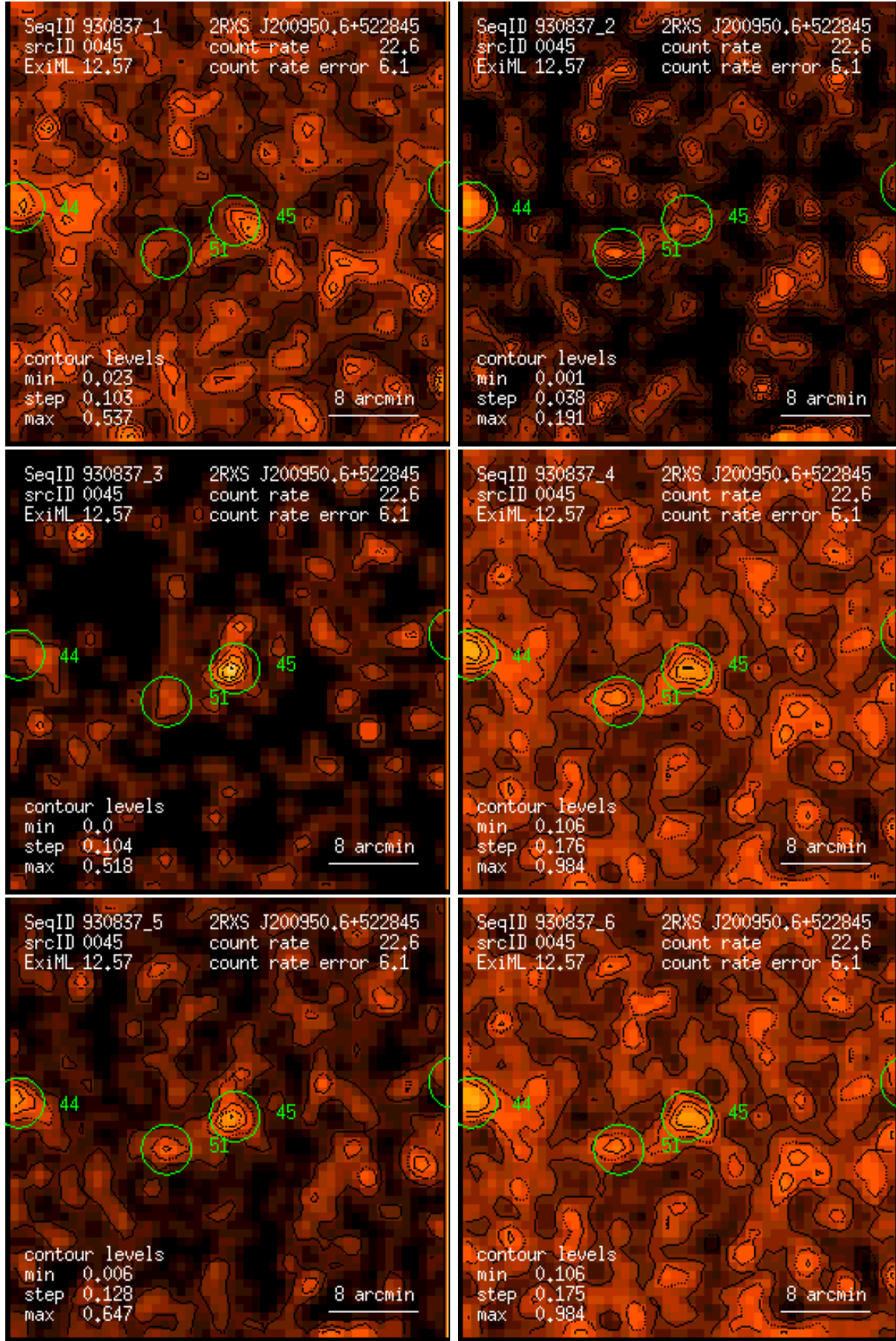
Figure 45: RASS 930837: detection 0045: band rate images, Gaussian filter: (1) PSPC channels 11 – 41, (2) 52 – 90, (3) 91 – 201, (4) 11 – 235, (5) 52 – 201, (6) 11 – 201. Broad band rates in counts/ks. Band rate contour levels in counts/ks/arcmin 2 .
