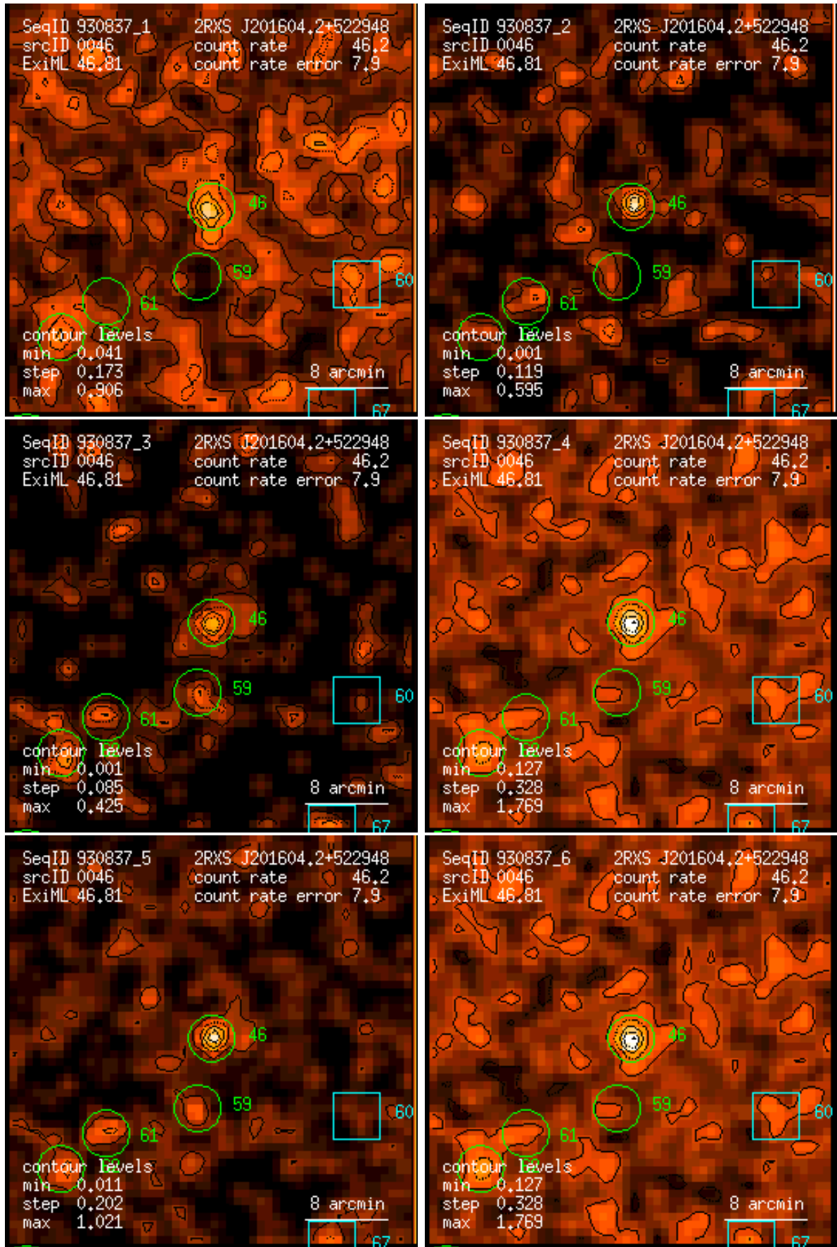
Figure 46: RASS 930837: detection 0046: band rate images, Gaussian filter: (1) PSPC channels 11 – 41, (2) 52 – 90, (3) 91 – 201, (4) 11 – 235, (5) 52 – 201, (6) 11 – 201. Broad band rates in counts/ks. Band rate contour levels in counts/ks/arcmin 2 .
