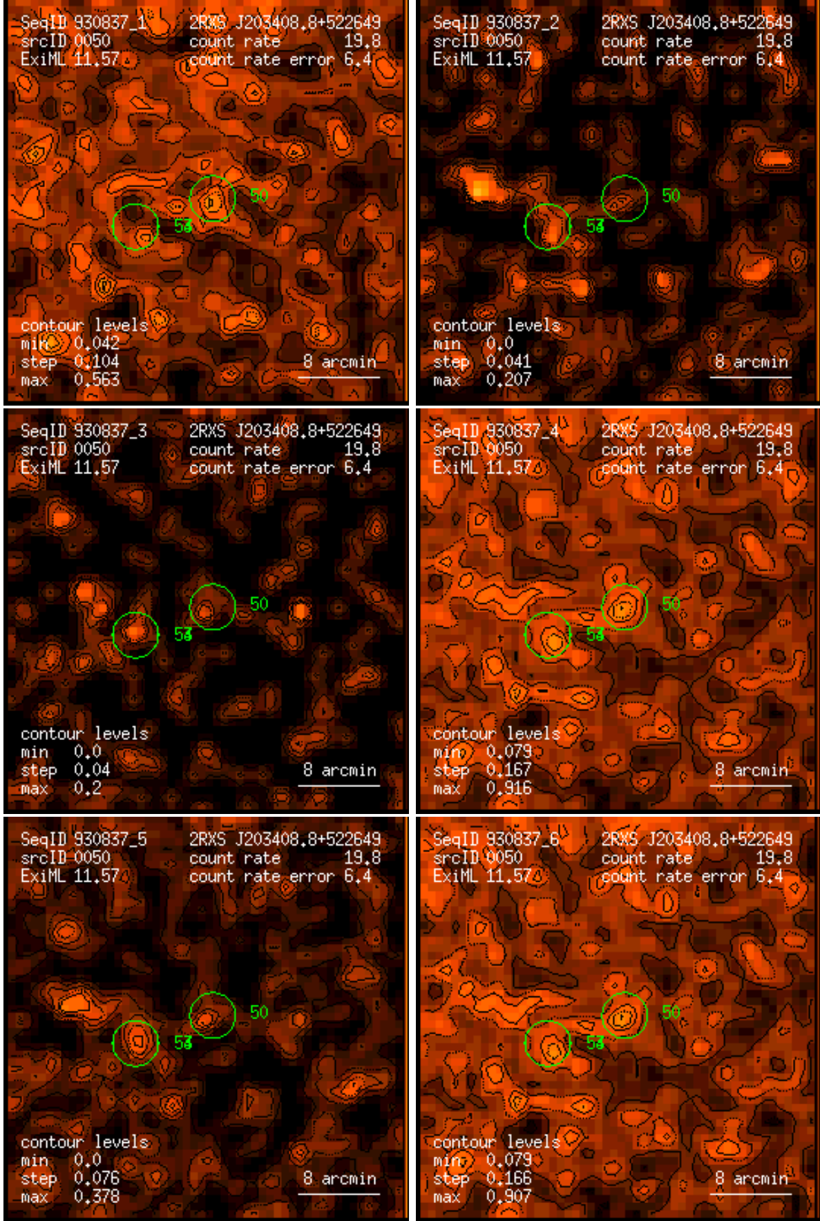
Figure 50: RASS 930837: detection 0050: band rate images, Gaussian filter: (1) PSPC channels 11 – 41, (2) 52 – 90, (3) 91 – 201, (4) 11 – 235, (5) 52 – 201, (6) 11 – 201. Broad band rates in counts/ks. Band rate contour levels in counts/ks/arcmin 2 .
