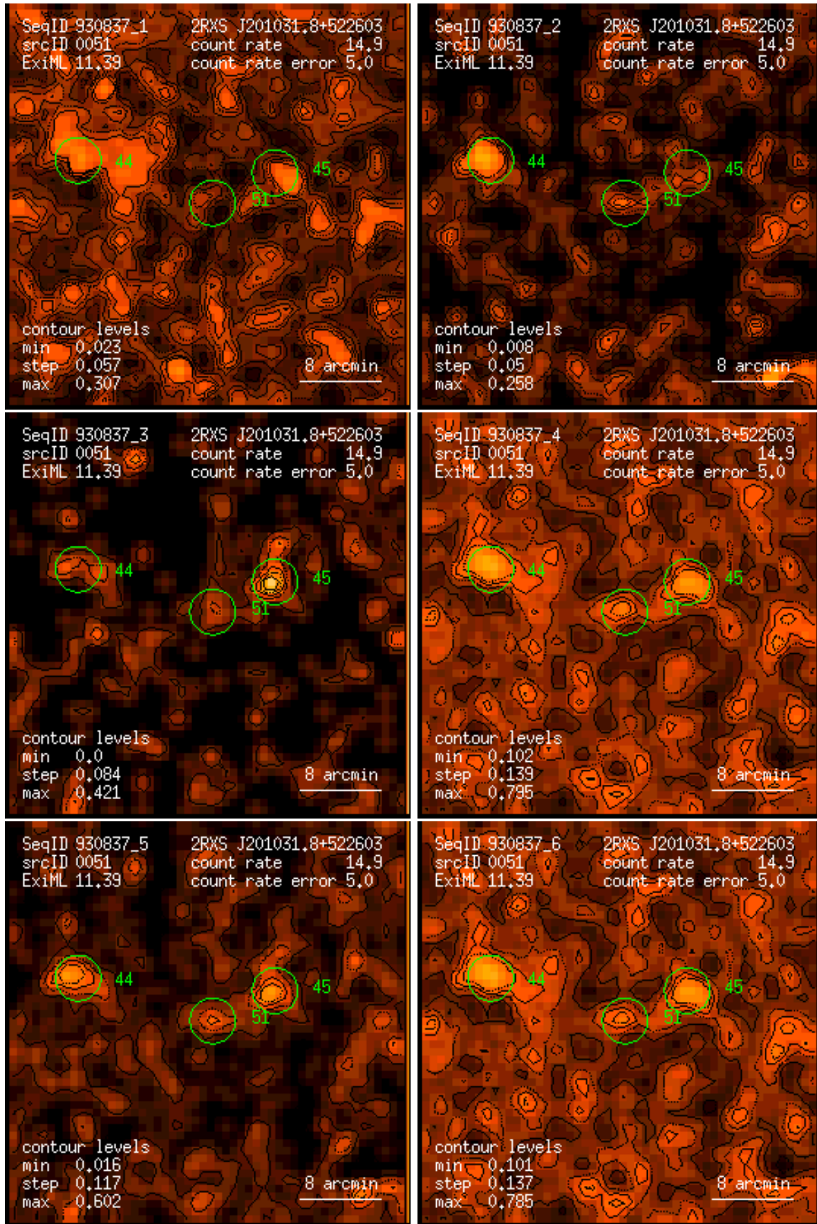
Figure 51: RASS 930837: detection 0051: band rate images, Gaussian filter: (1) PSPC channels 11 – 41, (2) 52 – 90, (3) 91 – 201, (4) 11 – 235, (5) 52 – 201, (6) 11 – 201. Broad band rates in counts/ks. Band rate contour levels in counts/ks/arcmin 2 .
