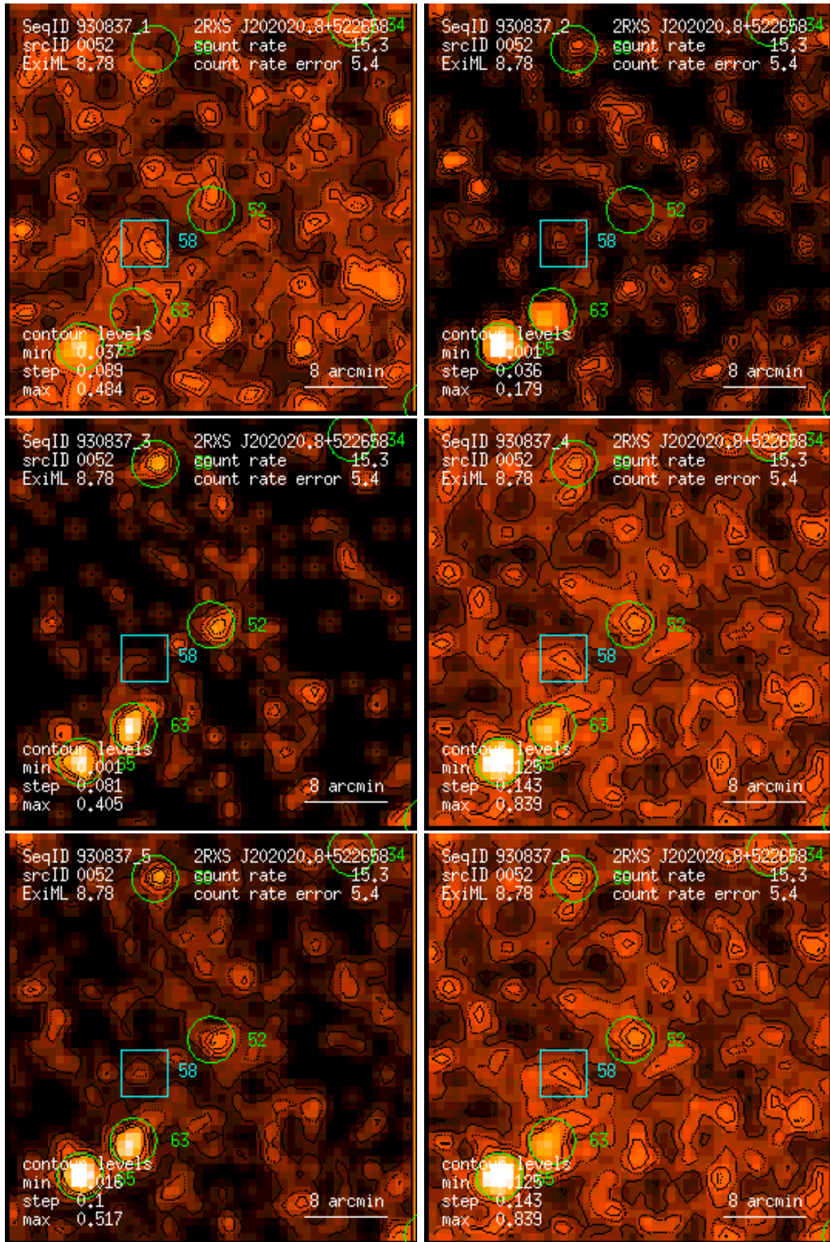
Figure 52: RASS 930837: detection 0052: band rate images, Gaussian filter: (1) PSPC channels 11 – 41, (2) 52 – 90, (3) 91 – 201, (4) 11 – 235, (5) 52 – 201, (6) 11 – 201. Broad band rates in counts/ks. Band rate contour levels in counts/ks/arcmin 2 .
