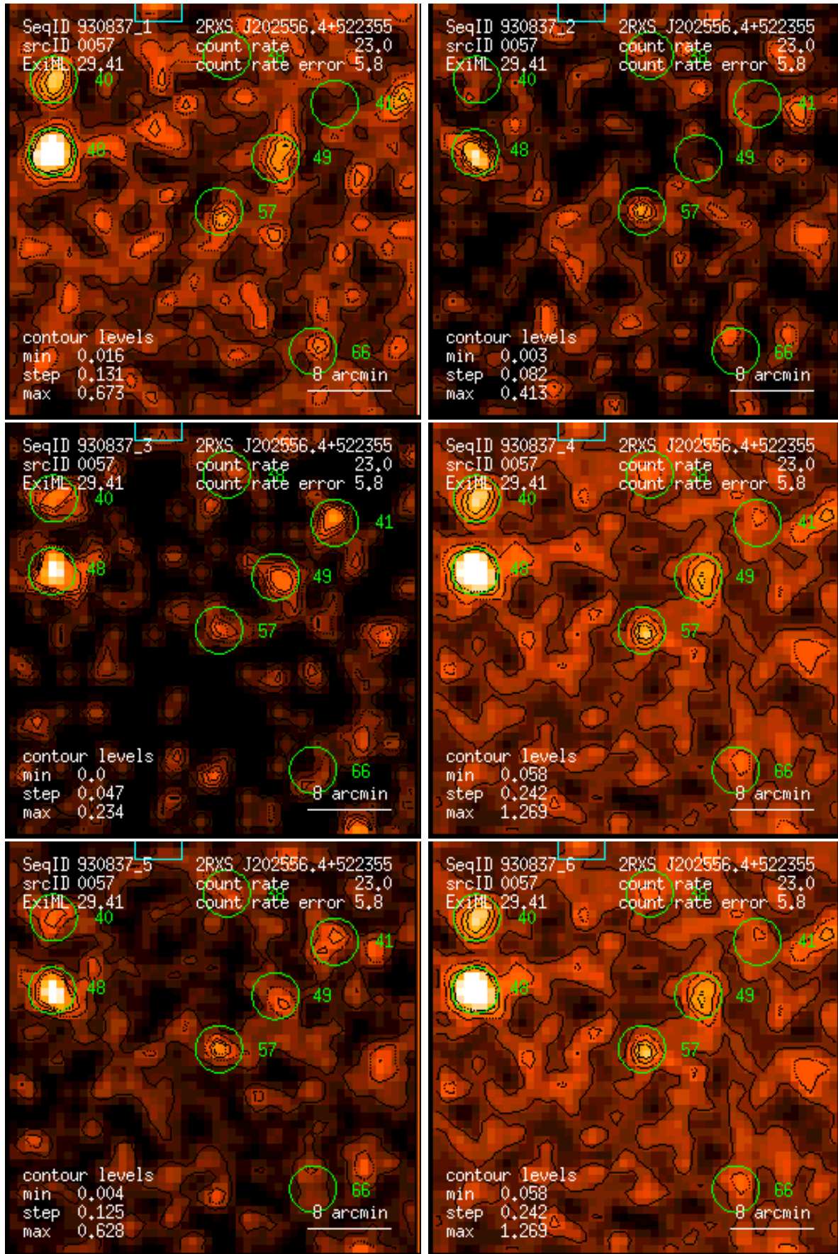
Figure 57: RASS 930837: detection 0057: band rate images, Gaussian filter: (1) PSPC channels 11 – 41, (2) 52 – 90, (3) 91 – 201, (4) 11 – 235, (5) 52 – 201, (6) 11 – 201. Broad band rates in counts/ks. Band rate contour levels in counts/ks/arcmin 2 .
