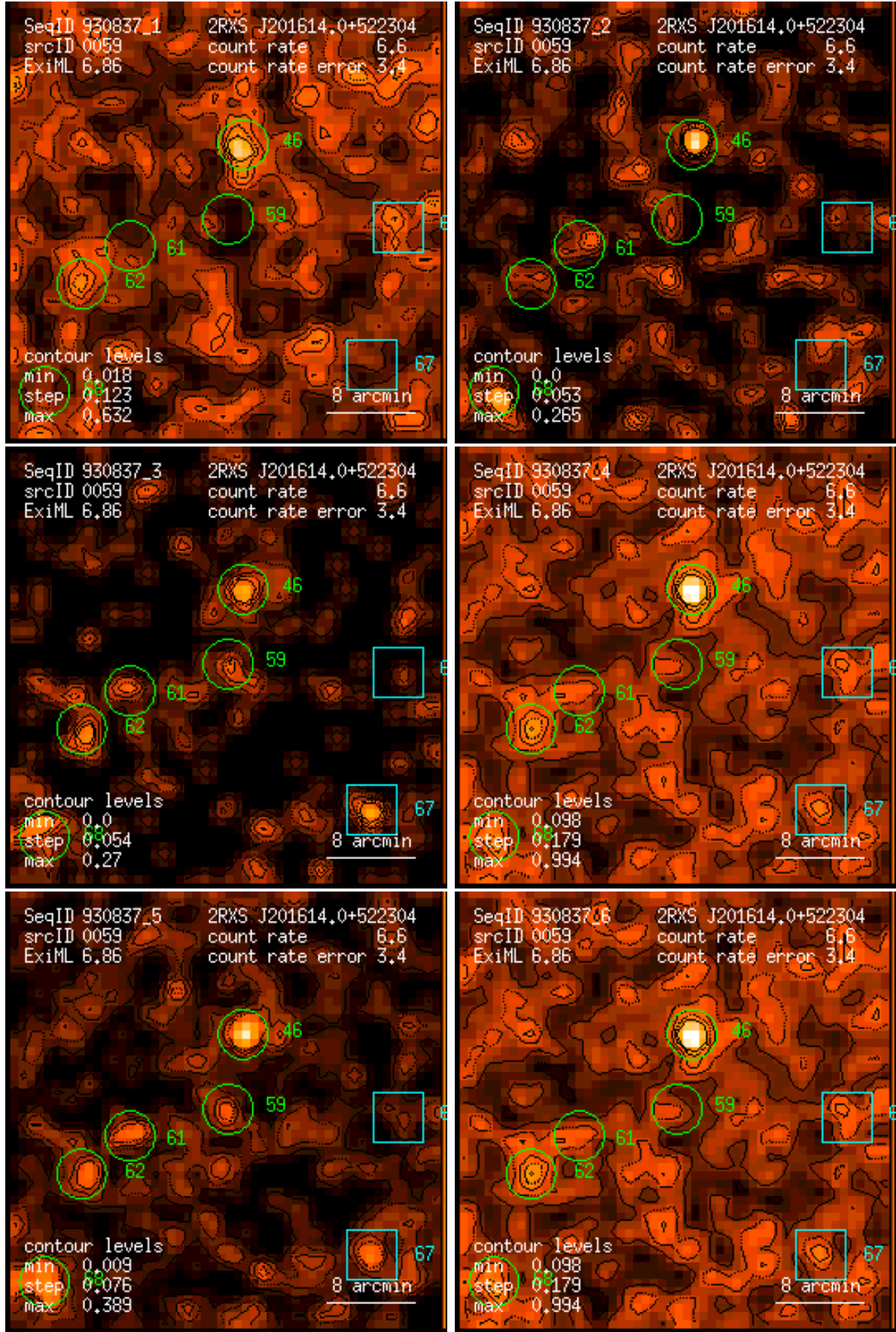
Figure 59: RASS 930837: detection 0059: band rate images, Gaussian filter: (1) PSPC channels 11 – 41, (2) 52 – 90, (3) 91 – 201, (4) 11 – 235, (5) 52 – 201, (6) 11 – 201. Broad band rates in counts/ks. Band rate contour levels in counts/ks/arcmin 2 .
