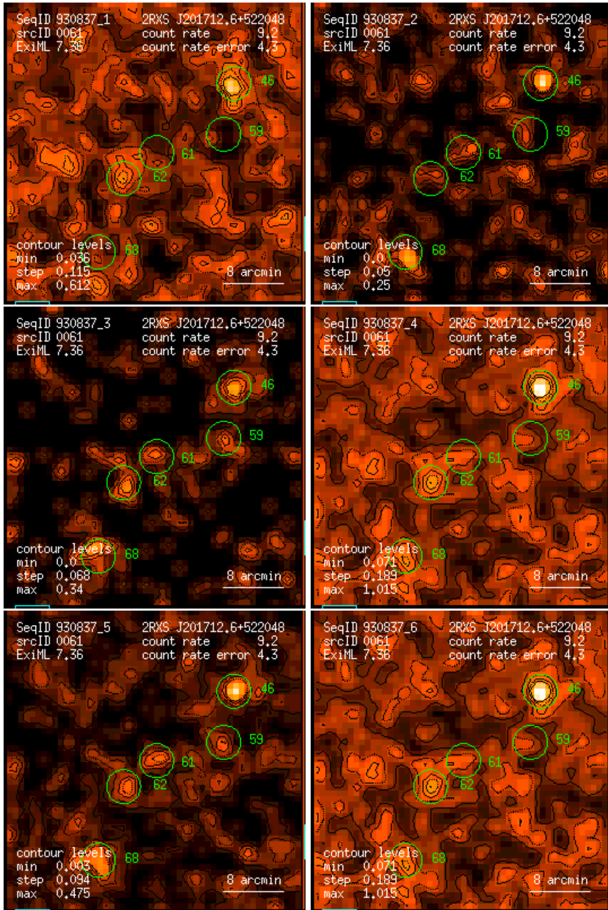
Figure 61: RASS 930837: detection 0061: band rate images, Gaussian filter: (1) PSPC channels 11 – 41, (2) 52 – 90, (3) 91 – 201, (4) 11 – 235, (5) 52 – 201, (6) 11 – 201. Broad band rates in counts/ks. Band rate contour levels in counts/ks/arcmin 2 .
