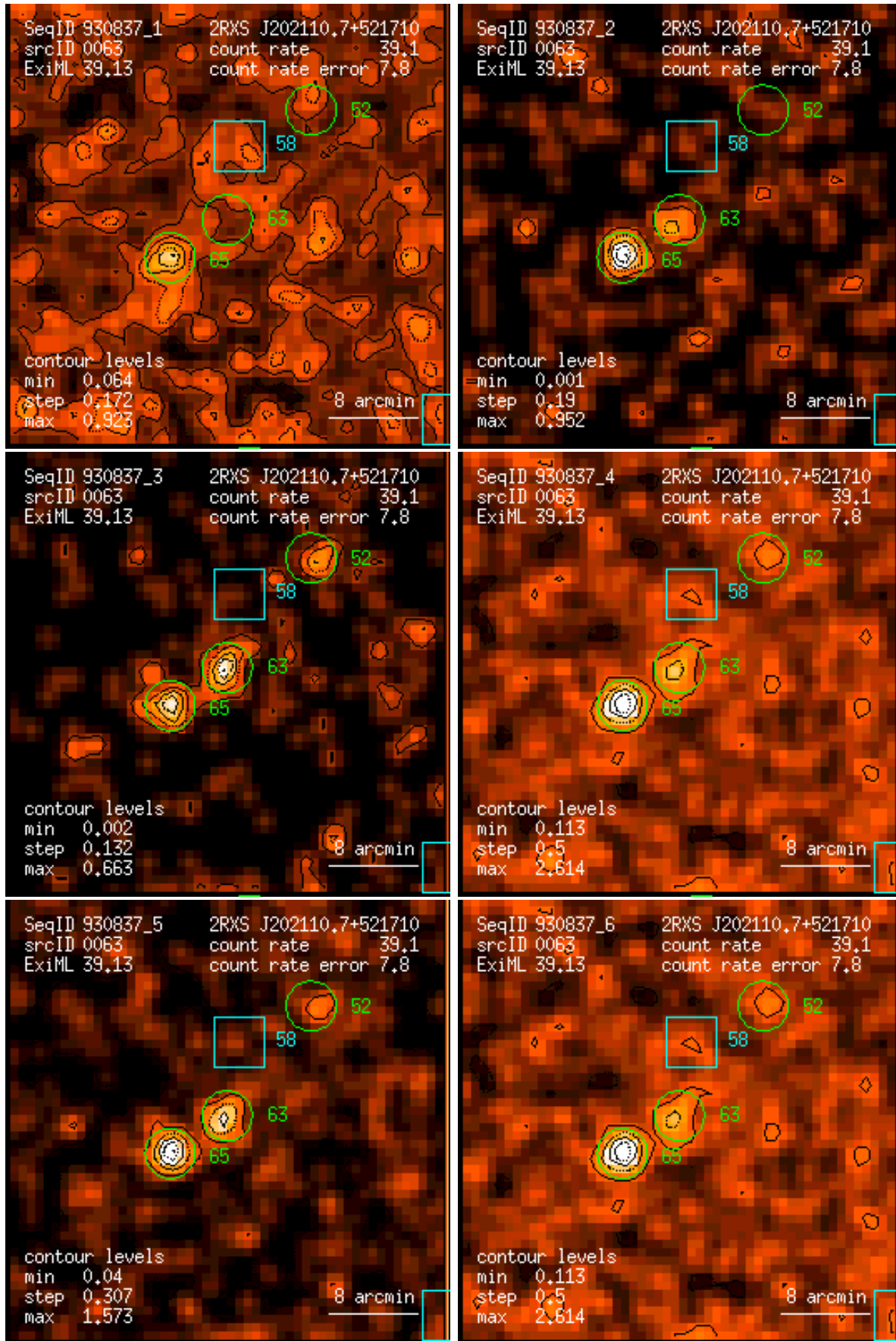
Figure 63: RASS 930837: detection 0063: band rate images, Gaussian filter: (1) PSPC channels 11 – 41, (2) 52 – 90, (3) 91 – 201, (4) 11 – 235, (5) 52 – 201, (6) 11 – 201. Broad band rates in counts/ks. Band rate contour levels in counts/ks/arcmin 2 .
