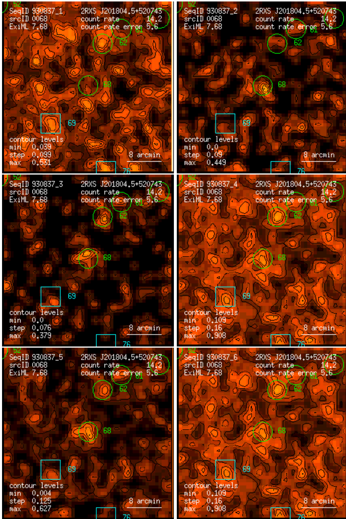
Figure 68: RASS 930837: detection 0068: band rate images, Gaussian filter: (1) PSPC channels 11 – 41, (2) 52 – 90, (3) 91 – 201, (4) 11 – 235, (5) 52 – 201, (6) 11 – 201. Broad band rates in counts/ks. Band rate contour levels in counts/ks/arcmin 2 .
