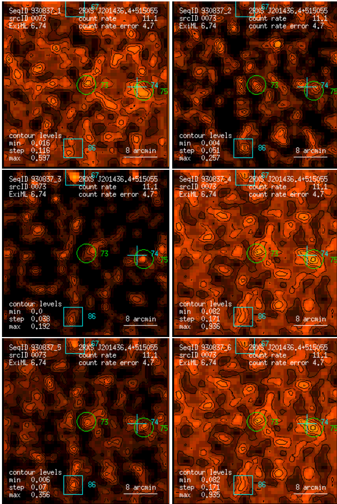
Figure 73: RASS 930837: detection 0073: band rate images, Gaussian filter: (1) PSPC channels 11 – 41, (2) 52 – 90, (3) 91 – 201, (4) 11 – 235, (5) 52 – 201, (6) 11 – 201. Broad band rates in counts/ks. Band rate contour levels in counts/ks/arcmin 2 .
