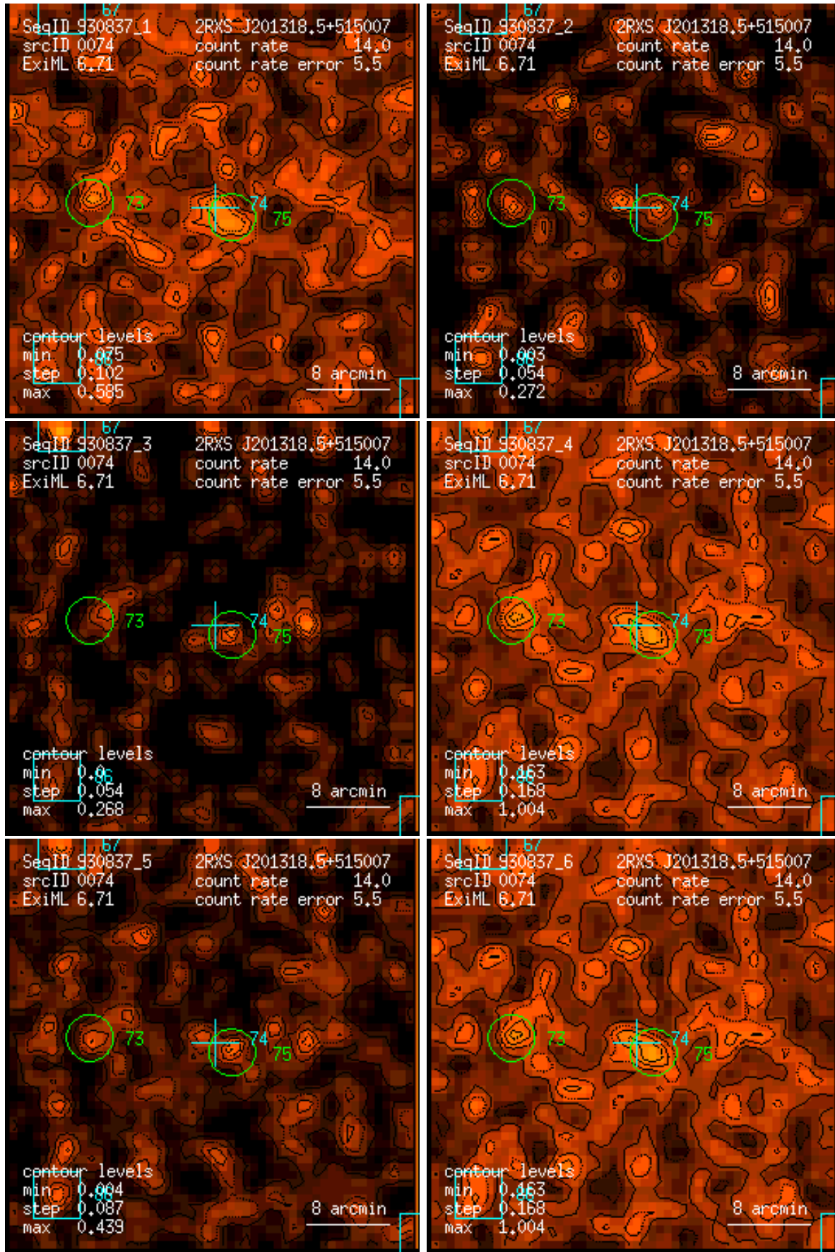
Figure 74: RASS 930837: detection 0074: band rate images, Gaussian filter: (1) PSPC channels 11 – 41, (2) 52 – 90, (3) 91 – 201, (4) 11 – 235, (5) 52 – 201, (6) 11 – 201. Broad band rates in counts/ks. Band rate contour levels in counts/ks/arcmin 2 .
