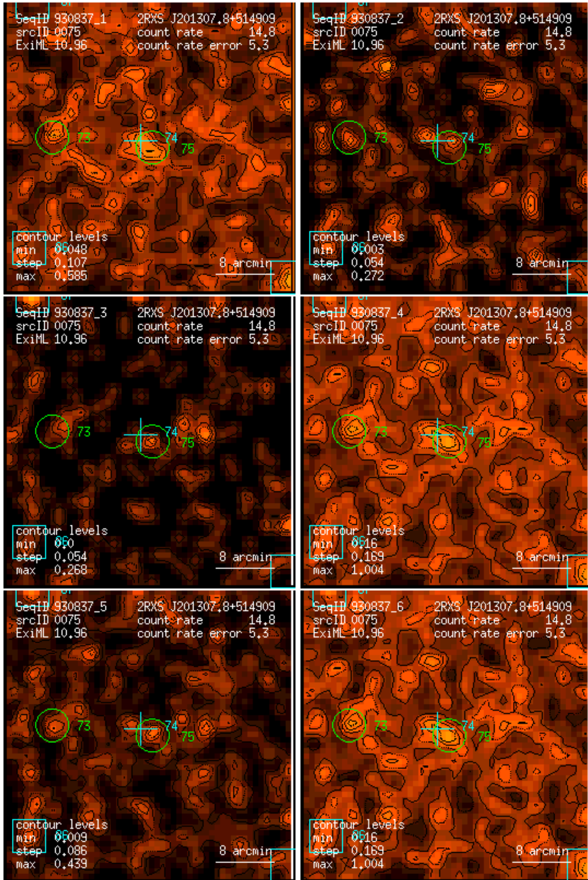
Figure 75: RASS 930837: detection 0075: band rate images, Gaussian filter: (1) PSPC channels 11 – 41, (2) 52 – 90, (3) 91 – 201, (4) 11 – 235, (5) 52 – 201, (6) 11 – 201. Broad band rates in counts/ks. Band rate contour levels in counts/ks/arcmin 2 .
